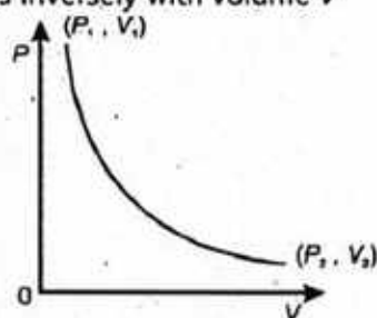
Fig. 1: Boyle's law
