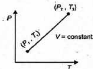
Fig. 3: Joseph Lussac's law
