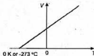
Fig. 2: Charles' law
