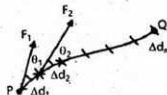
Fig. 5: A particle acted upon by a variable force, moves along the path shown from point P to point Q.
