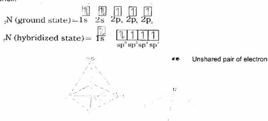
Figure 3.10: Structure of Ammonia ( NH_3 )
