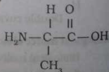
Alanine
