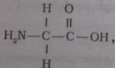
Glycine
