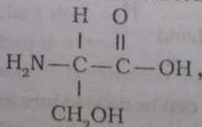
Serine
