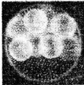
Figure 1.5 volvox colony
