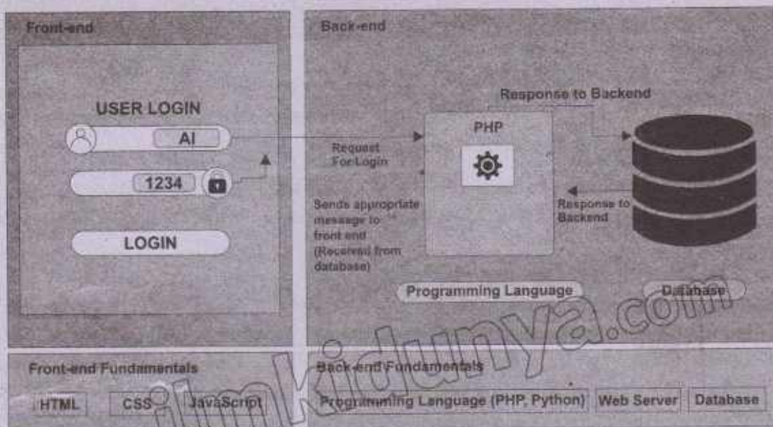
Graphical abstract of login system
