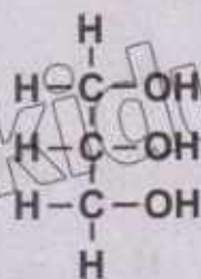
Glycerol
