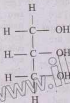
Glycerol
