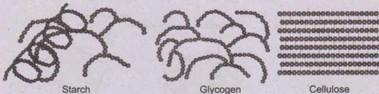
Figure 6.4: Polysaccharides
