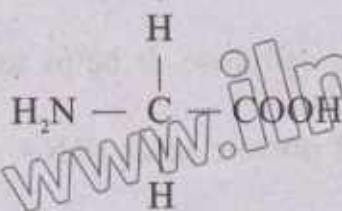
Glycine
