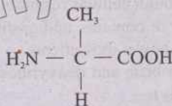
Alanine
