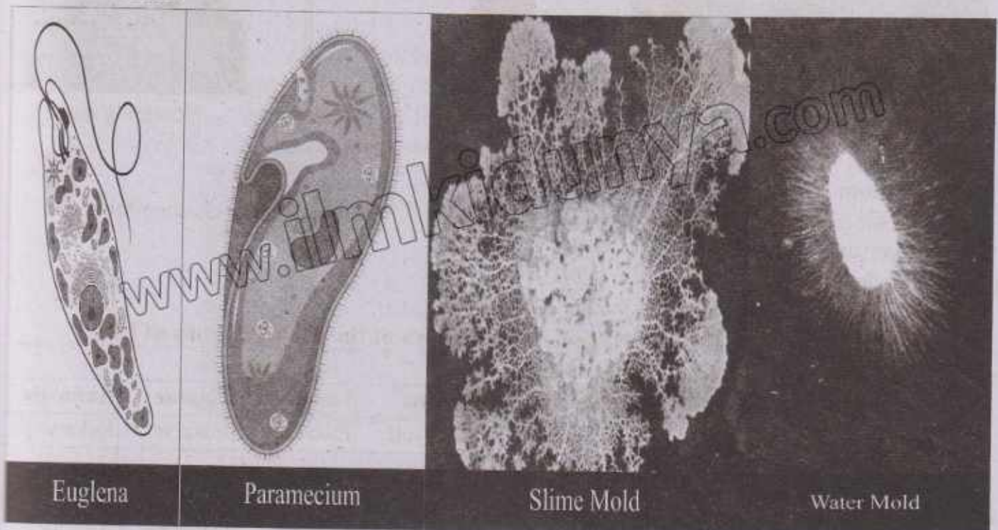
Figure 2.5: Common Protists
