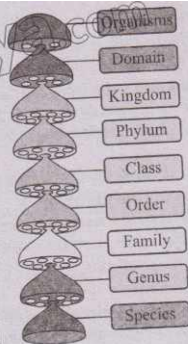
Figure 2.1: Taxonomic Ranks
