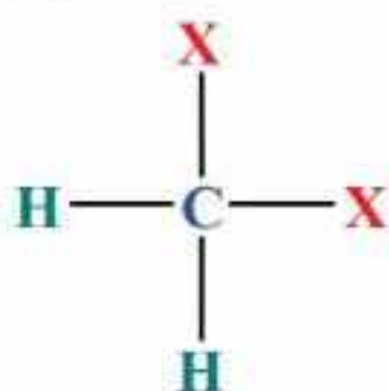
Dihalogenoalkane
