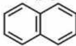
Napthalene C_{10}H_8
