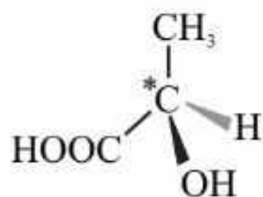
(-) lactic acid
