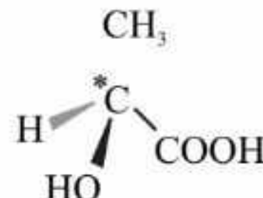
(+) lactic acid
