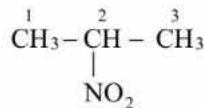
2-nitropropane
