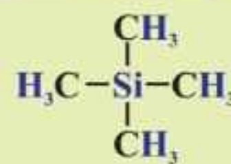
Tetramethylsilane (TMS)
