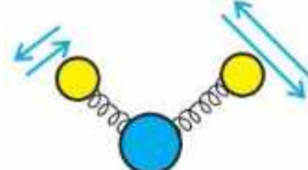
Asymmetric Bending
