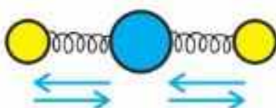
Symmetric Stretching
