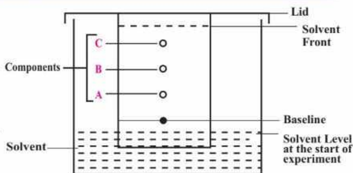
Figure 28.2 Paper Chromatography
