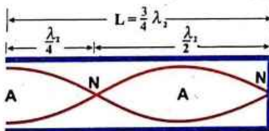
Fig.8.22: Second Harmonic stationary wave with one and half loops have two nodes and two anti-nodes.
