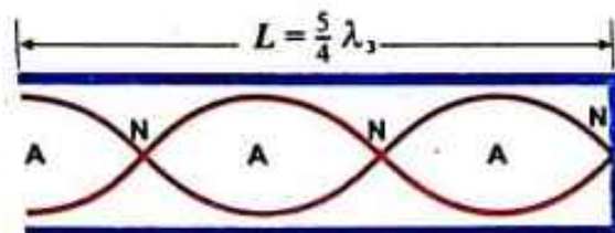
Fig.8.23: Third Harmonic stationary wave with two and half loops have three nodes and three anti-nodes.
