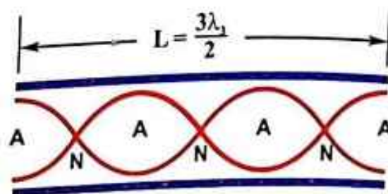
Fig.8.26: Third Harmonic
