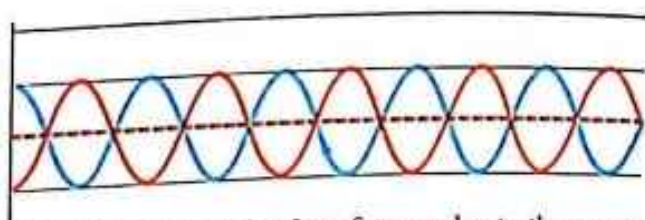
Fig.8.12: Destructive Interference due to the superposition of coherent waves, in the opposite phase.
