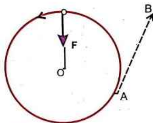
Fig.5.10: The ball moving outward
