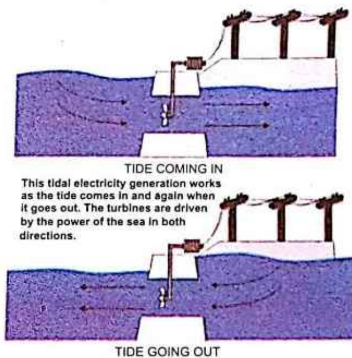
Fig.4.32: Tidal Energy
