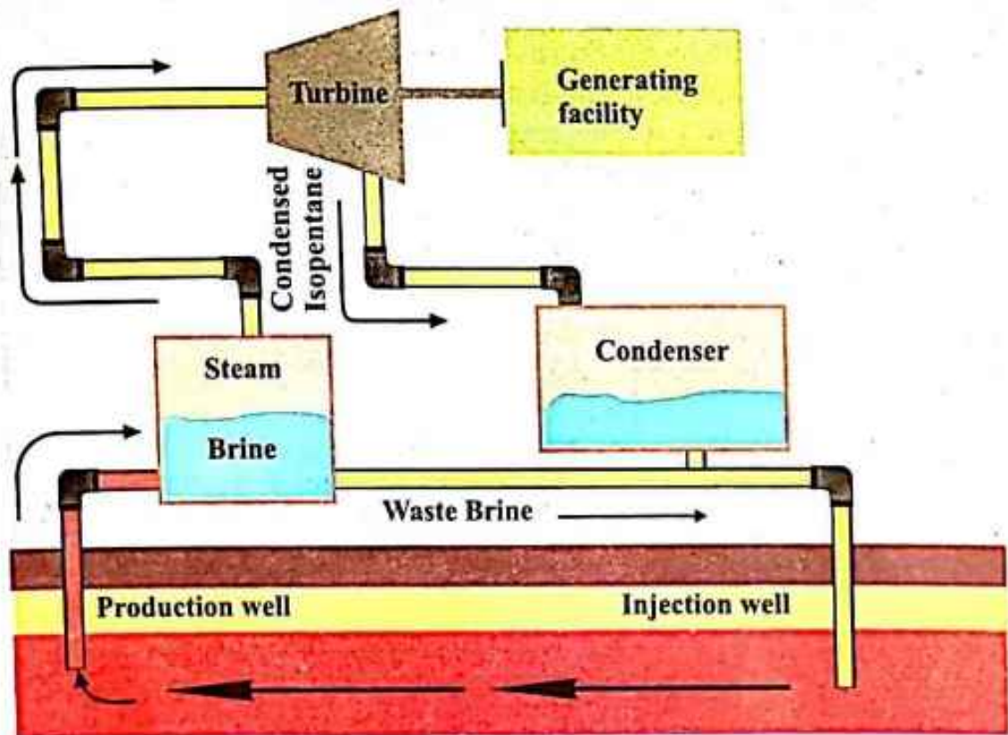
Fig.4.30: Geothermal Energy
