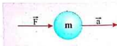
Fig.3.15: Acceleration in the direction of force
