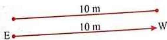
Fig.3.1: Distance vs. Displacement
