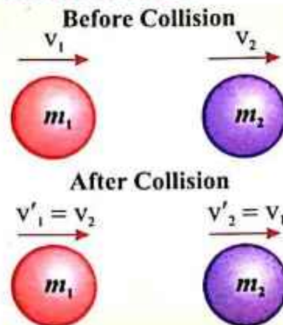
Fig.3.25: One dimension elastic collision of two bodies where m_1 = m_2 .
