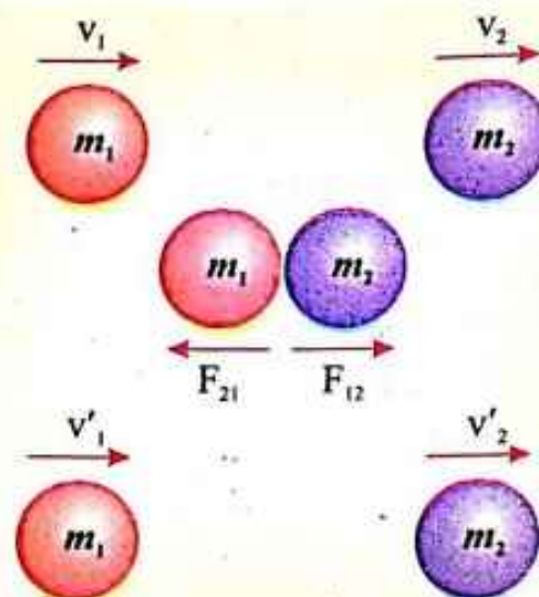
Fig.3.23: Collision of spheres which follows the law of conservation of momentum
