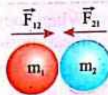
Fig.3.17: Two bodies exert the forces on each other which are same in magnitude but act in opposite directions.
