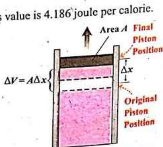
Fig.10.4: Work done by a system due to the expansion of volume by reducing the pressure.
