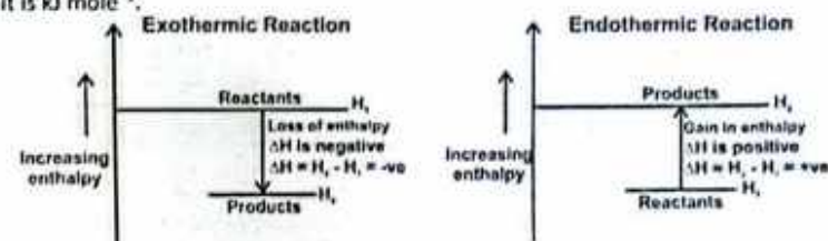
Enthalpy changes in thermochemical reactions
