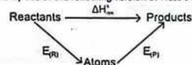
Figure: Hess Cycle; showing the relationship between B.E.'s and \Delta H_r = \sum nE_R - \sum nE_P
