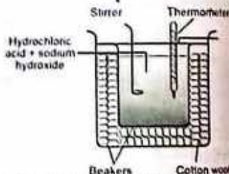
Figure: Glass calorimeter to measure enthalpy change of reactions
