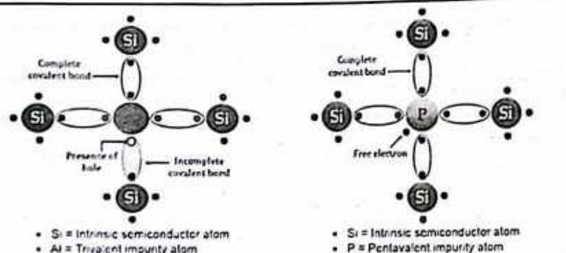
Formation of P type extrinsic semiconductor
