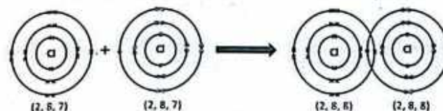
Figure: formation of a covalent bond between two Cl atoms
