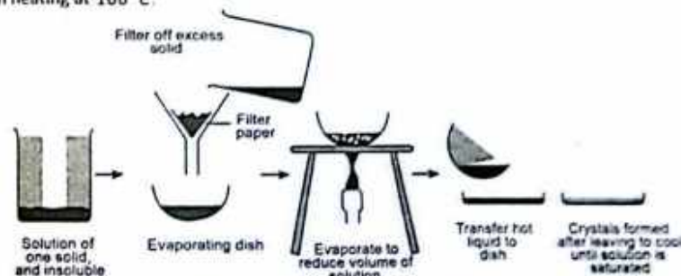
Figure: Different steps involved in crystallization
