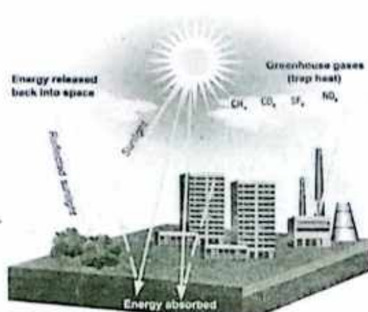
Figure: Mechanism of Global Warming
