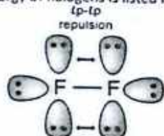
Figure: F 2 molecule with lone pairs of electrons
