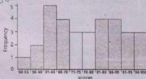
Figure : Histogram showing the distribution of exam scores
