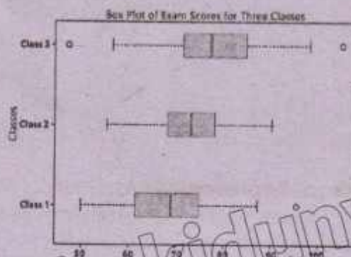
Figure : A Boxplot, showing class scores performance of three classes
