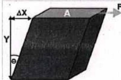
Shear Modulus
