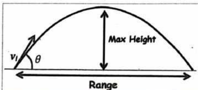
Figure 3.5: Height and range of a projectile.
