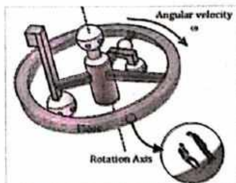
Figure 4.22: Artificial gravity.
