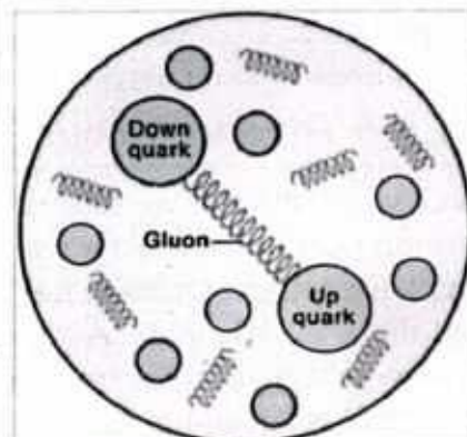
Figure 14.15: exchange of gluon between two quarks.
