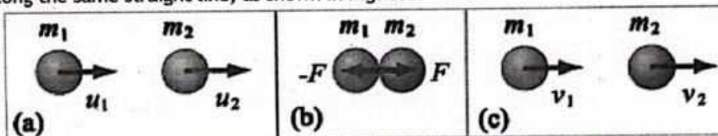
Figure 3.9: Two balls: (a) before collision (b) during collision (c) after collision.
