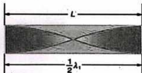
Figure 9.9 (a): Fundamental Frequency
