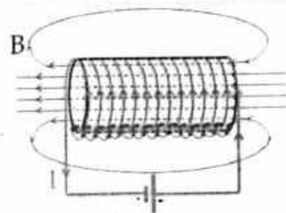
Figure 12.15: Solenoid.
