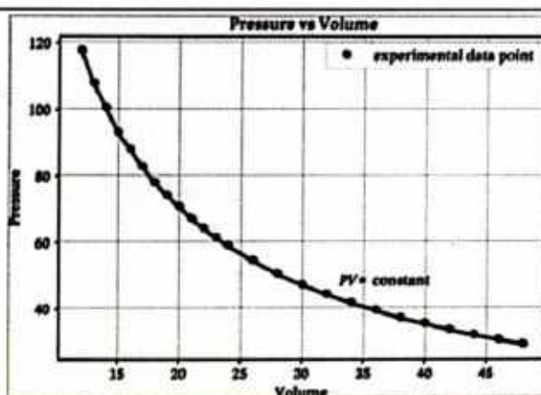
Figure 8.7: Boyle's law.
