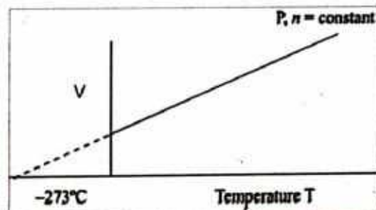
Figure 8.8: Charles's law.
