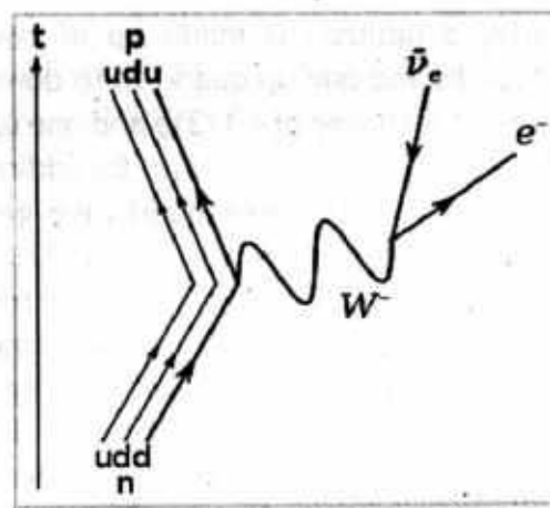
Figure 14.11: Beta-negative decay.
