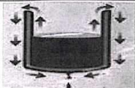
Figure 6.16: Super fluids creeps over the walls of containers to 'empty' themselves.
