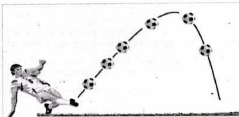
Figure 3.2: Two-dimensional motion of a football.
