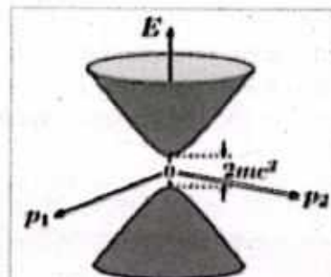
Figure 14.1: Electron-positron energy.
