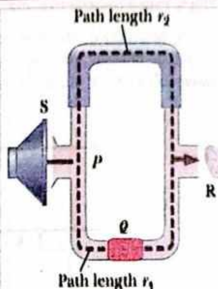
Figure 9.5 (a): Interference of Sound.
