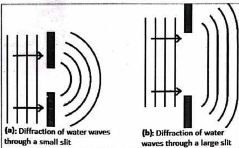
Figure 9.12: For observable diffraction separation between obstacles must be equal to the wavelength.
