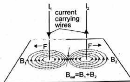
(b) currents in opposite direction - repulsive forces
