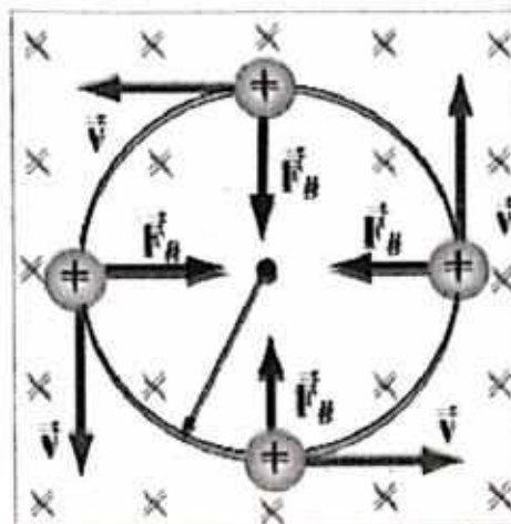
Figure 12.11: A magnetic force acts on charged particle and move it into a circular path.
