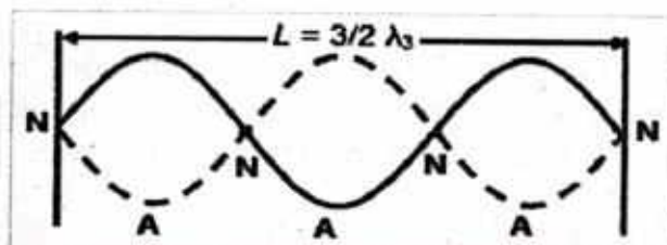
Figure 9.8 (d): Stationary wave having three loops.
