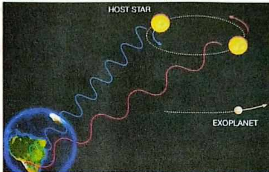
Figure 9.2: Blue shift and red shift.
