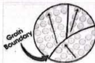
Figure 7.2: Polycrystalline structure.
