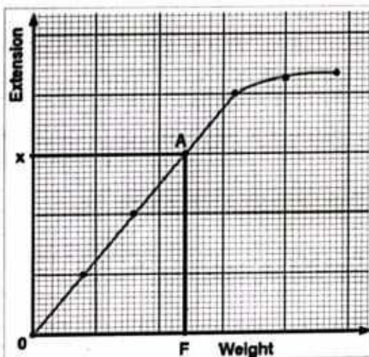
Figure 7.14: Force-extension graph.
