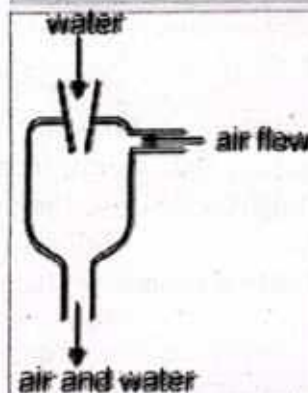
Figure 6.11: Filter pump.
