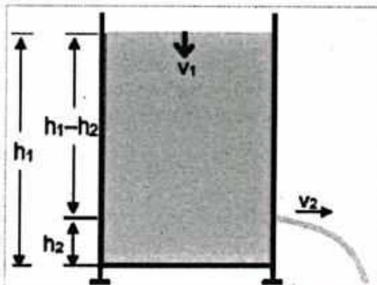
Figure 6.12: A tank filled with water and has an orifice near the bottom. The top surface of water comes down with almost zero speed.
