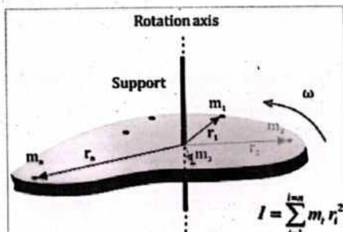
Figure 4.15: Rigid body rotating about axis of rotation.
