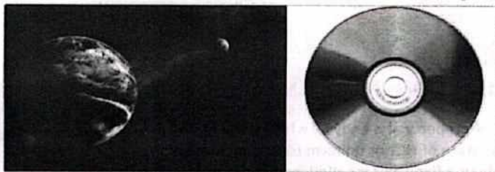
Figure 4.10 (d): Examples of centripetal force.
