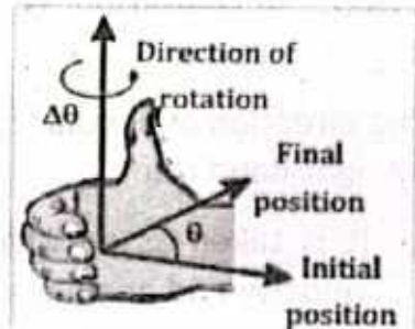
Right Hand Rule
