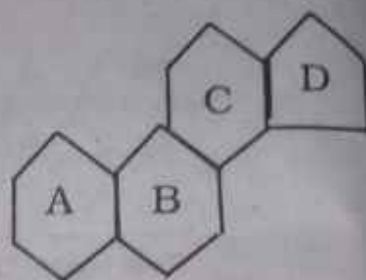
Fig. 2.8 Steroid nucleus
