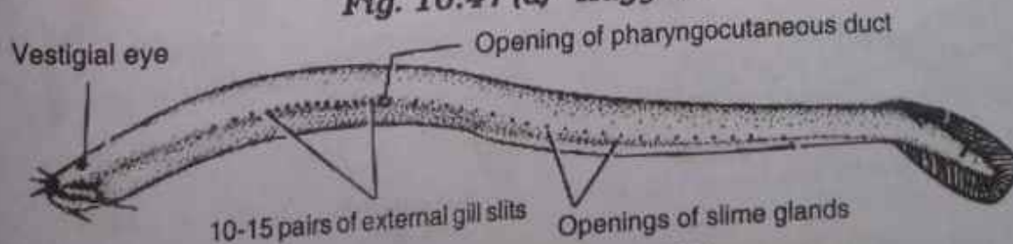
Fig. 10.47 (b) Lamprey
