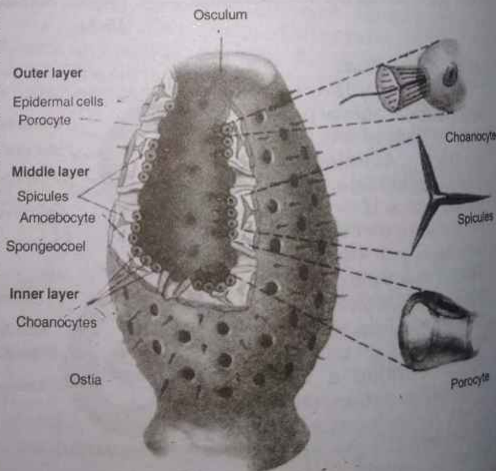
Fig. 10/7 Spongocoel
