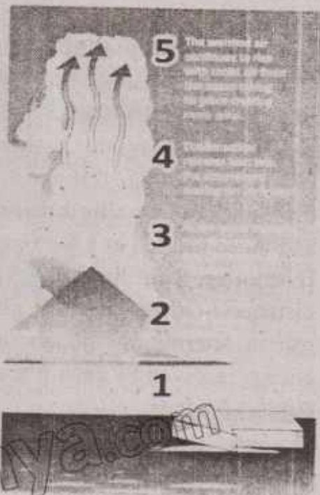
Fig. 21.4: Formation of Cyclone
