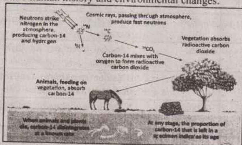
Fig. 20.15: Carbon dating
