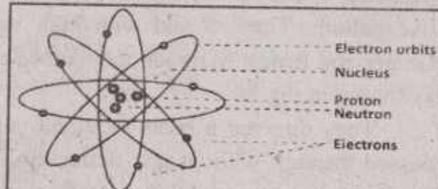
Fig. 20.2: Diagram of an atom showing the nucleus, protons, neutrons, and electron orbits
