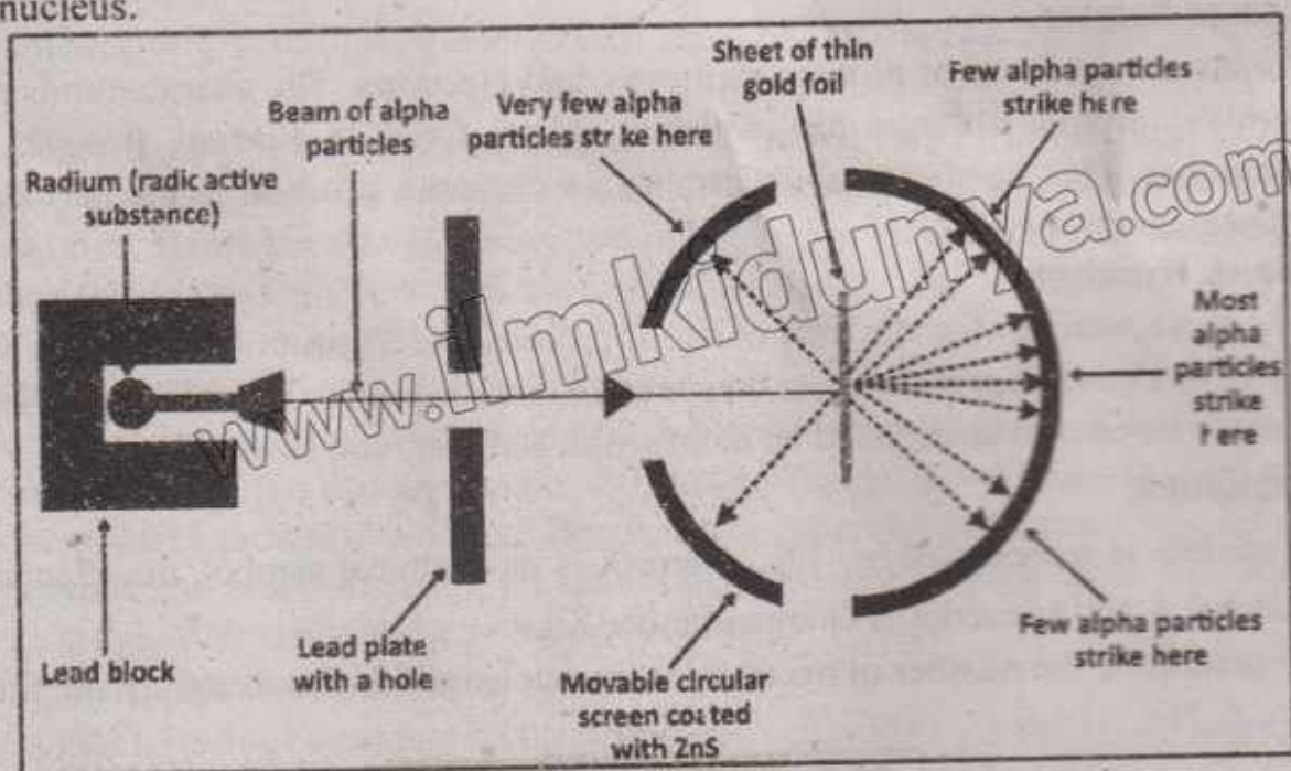
Fig. 20.1: Rutherford's gold foil experiment: scattering of alpha particles
