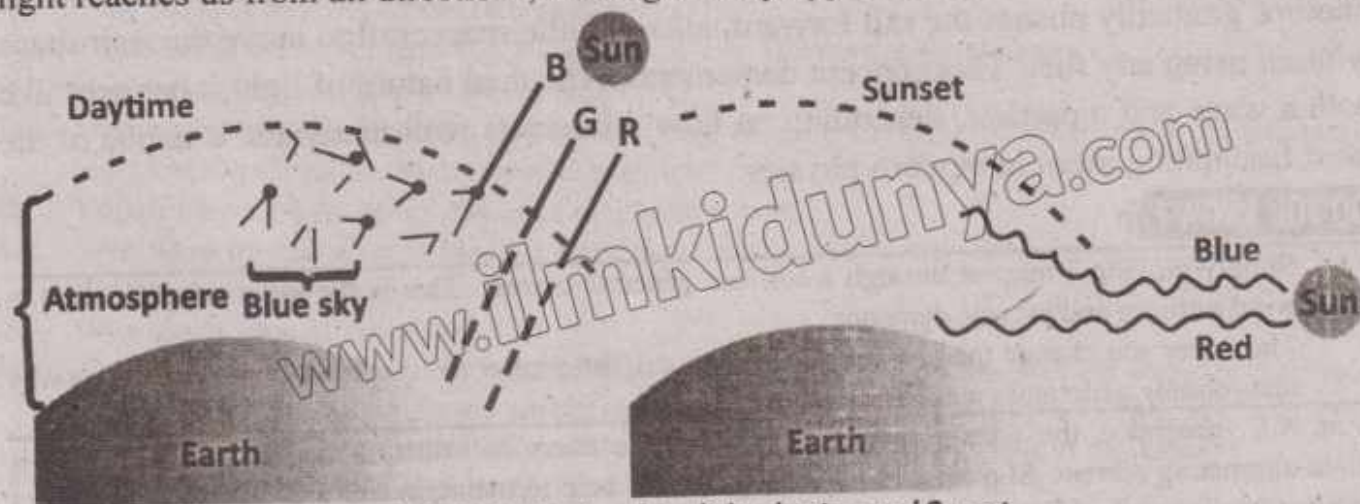
Fig 18.13: Scattering of Sunlight daytime and Sunset
