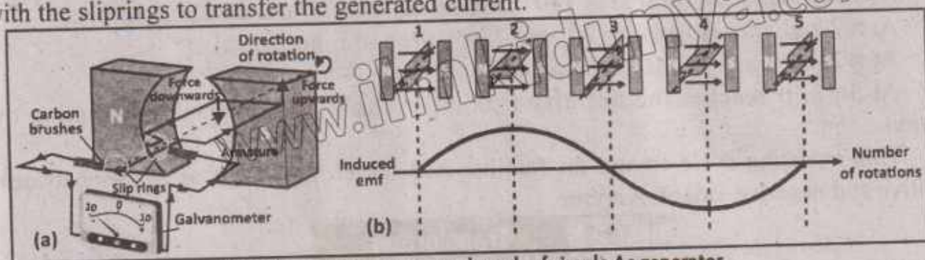
Fig. 18.5: An AC generator and graph of simple AC generator
