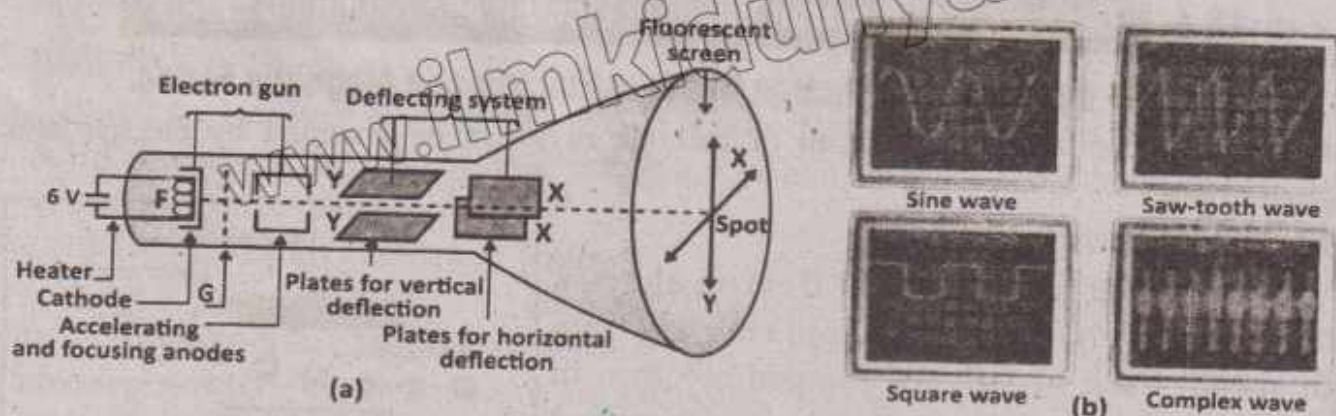
Fig 18.11: (a) Schematic diagram of CRO (b) Different waveforms displayed on a CRO screen
