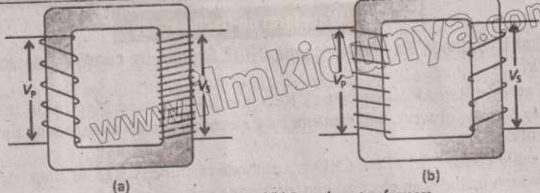
Fig 18.8: (a) Step-up and (b) Step-down transformers
