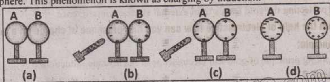
Fig. 15.5: Charging two spheres electrostatic induction
