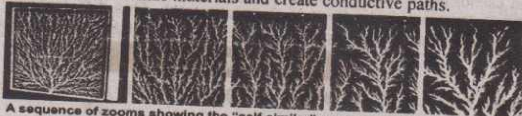
Fig.15.18: Self-Similarity in lichtenberg figures
