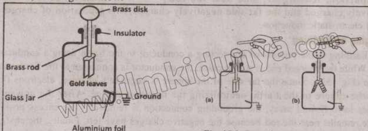
Fig. 15.7: Unchanged electroscope
