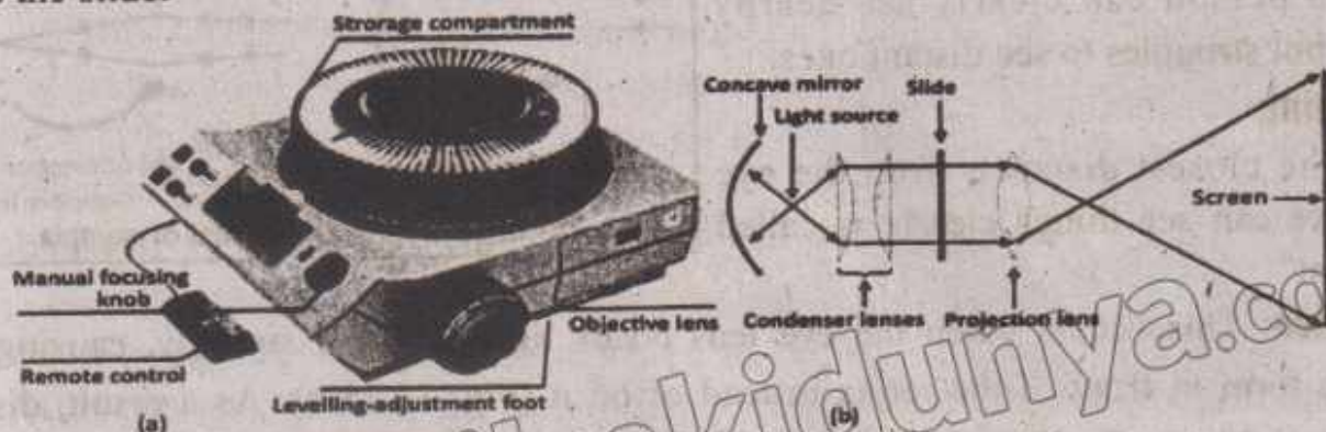
Fig. 14.22: (a) Slide projector (b) Ray diagram of slide projector
