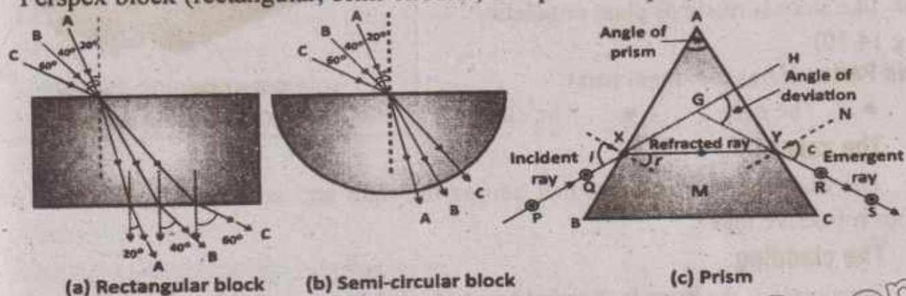
Fig. 14.8: Experiment for refraction of light
