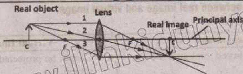
Fig. 14.17: Image formation by a convex lens
