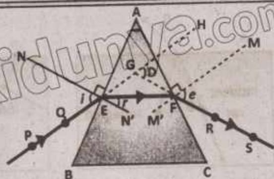
Fig. 14.6: Refraction through a triangular glass prism
