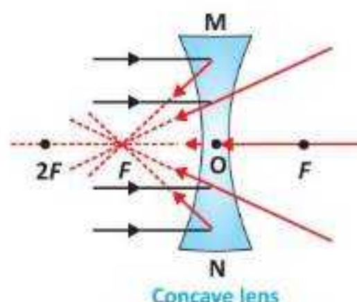
Fig. 14.16: Action of concave lens on parallel rays
