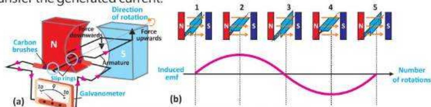
Fig. 18.5: An A.C generator and graph of current
