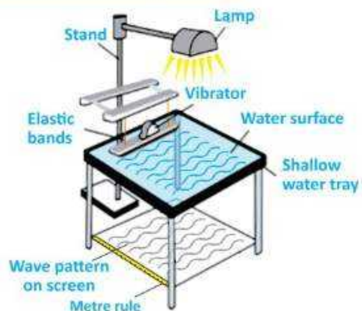
Fig. 12.5: Ripple tank
