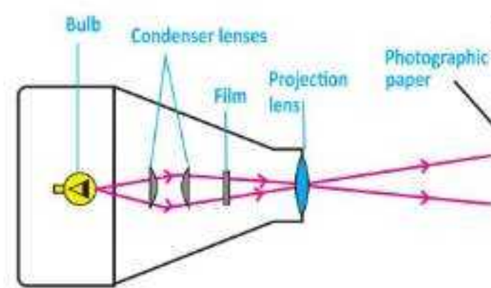
Fig. 14.23: Diagram of photograph enlarger
