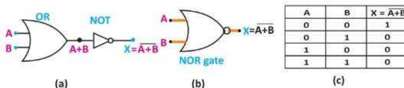
Fig. 19.18 (a,b): The circuit symbol (c) Truth table for NOR gate
