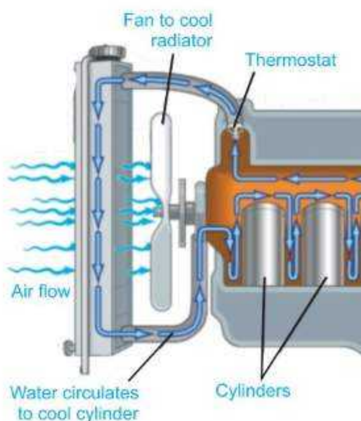
Fig. 10.7: Cooling system of automobile
