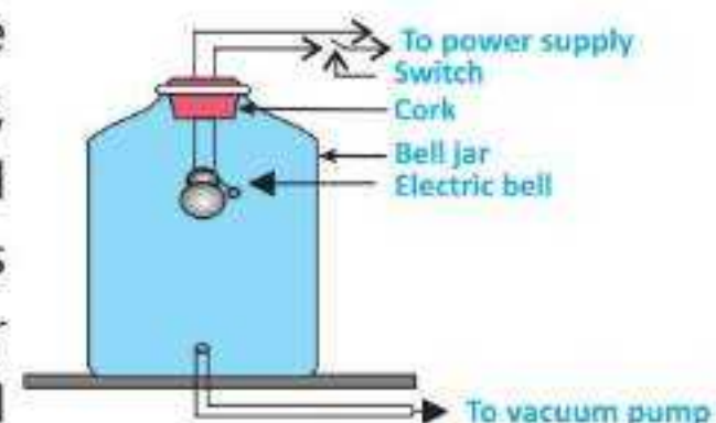
Fig.13.5: Bell jar apparatus
