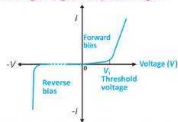
Fig. 19.5: I - V graph of a semiconductor diode
