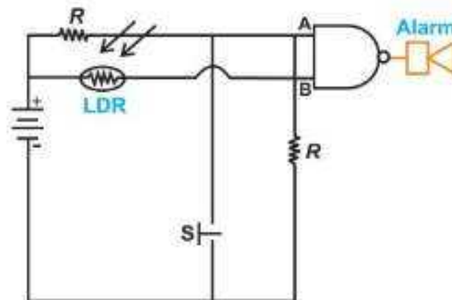
Fig. 19.19: Burglar alarm circuit using NAND gate
