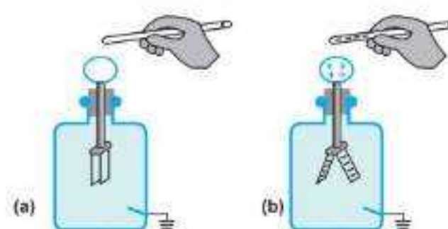
Fig. 15.8: Detecting charge using a gold leaf electroscope
