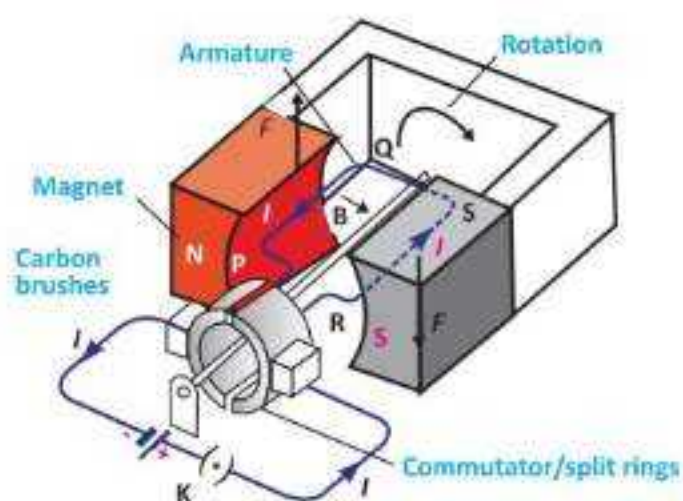
Fig. 17.9: Working principle of D.C motor
