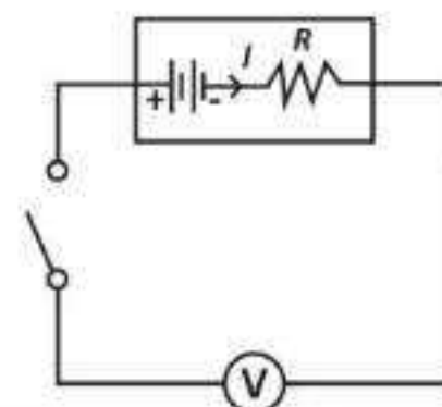
Fig. 16.5: Schematic diagram for measuring e.m.f. of the battery
