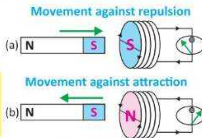
Fig. 18.4: Lenz's law
