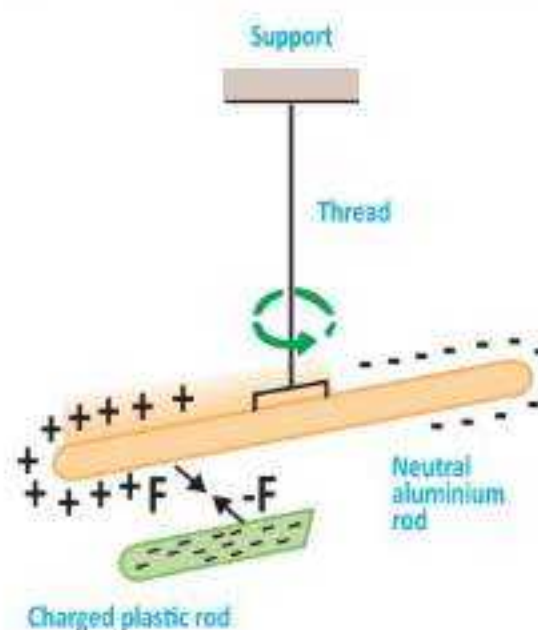
Fig. 15.4: Charged plastic rod attracts neutral aluminium rod
