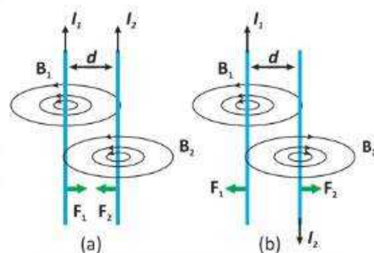
Fig. 17.5: Forces between parallel wires
