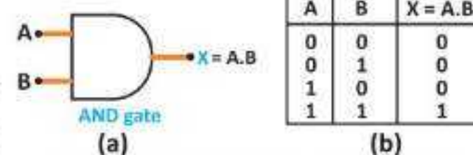
Fig. 19.14: (a) The circuit symbol and (b) Truth table for an AND gate
