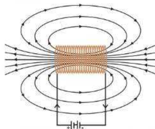
Fig. 17.3: Magnetic field due to solenoid
