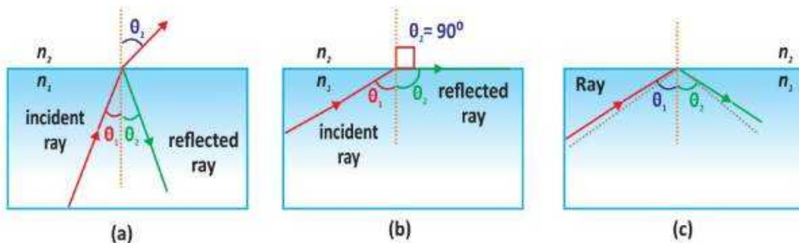
Fig. 14.7: Total internal reflection
