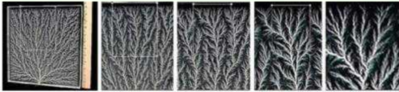
A sequence of zooms showing the "self-similar" property of lichtenberg figures
