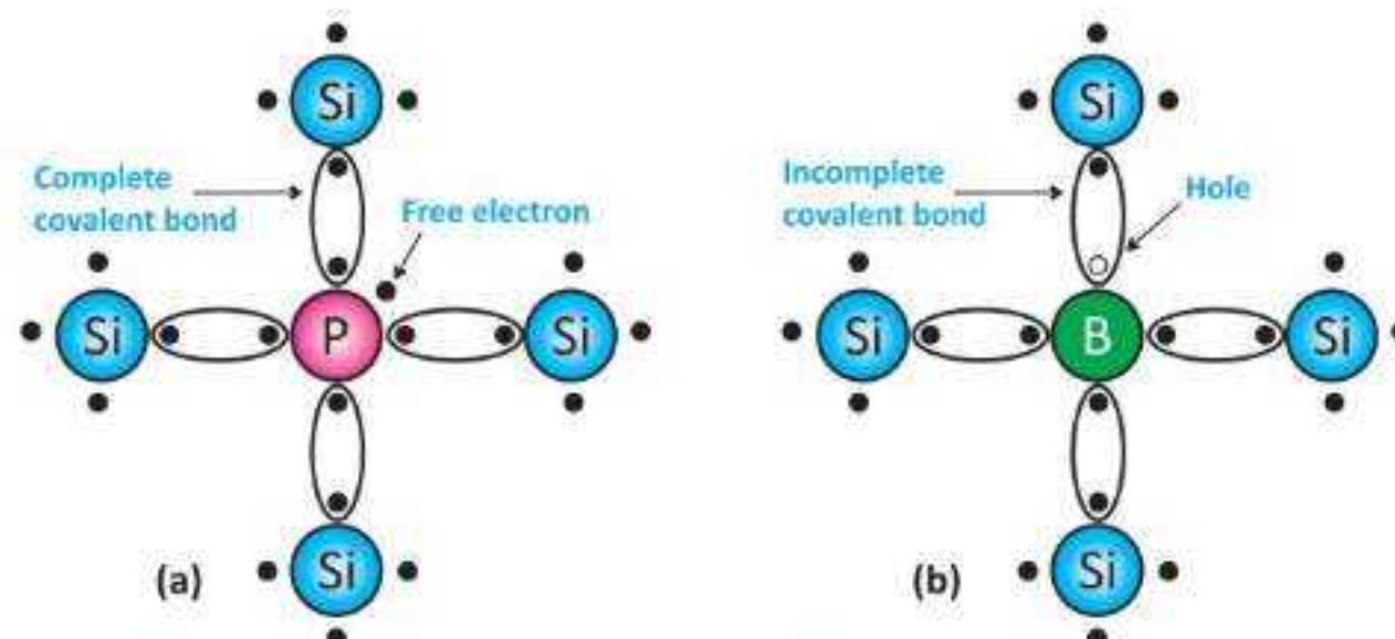
Fig. 19.1: (a) N-type semiconductors (b) P-type semiconductors
