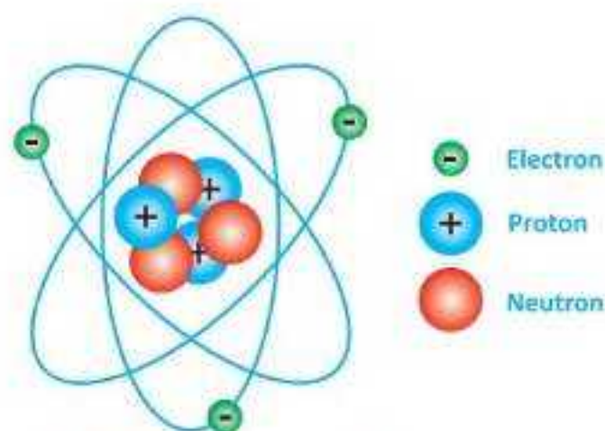
Fig. 15.3: Structure of an atom
