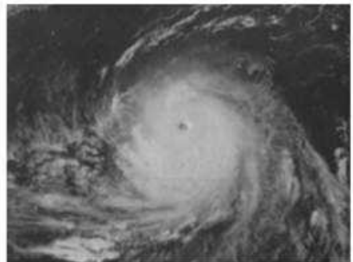
Fig. 21.6: Hurricane
