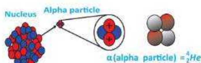
Fig. 20.4: Representing alpha particle
