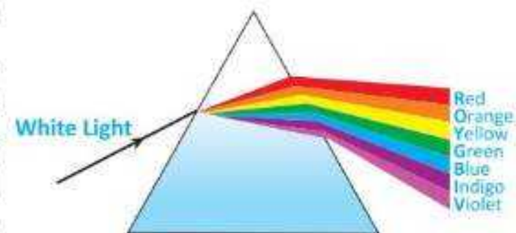
Fig. 14. 29: Dispersion of light by prism
