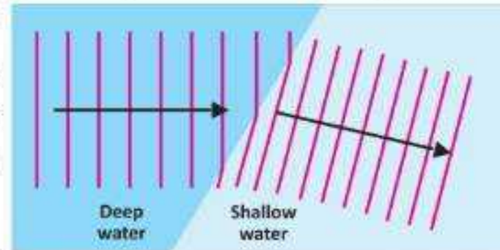
Fig. 12.12: Refraction of waves
