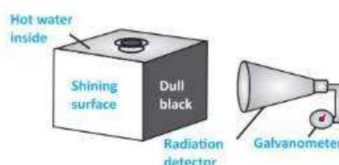
Fig. 11.11: Radiations from Leslie's cube
