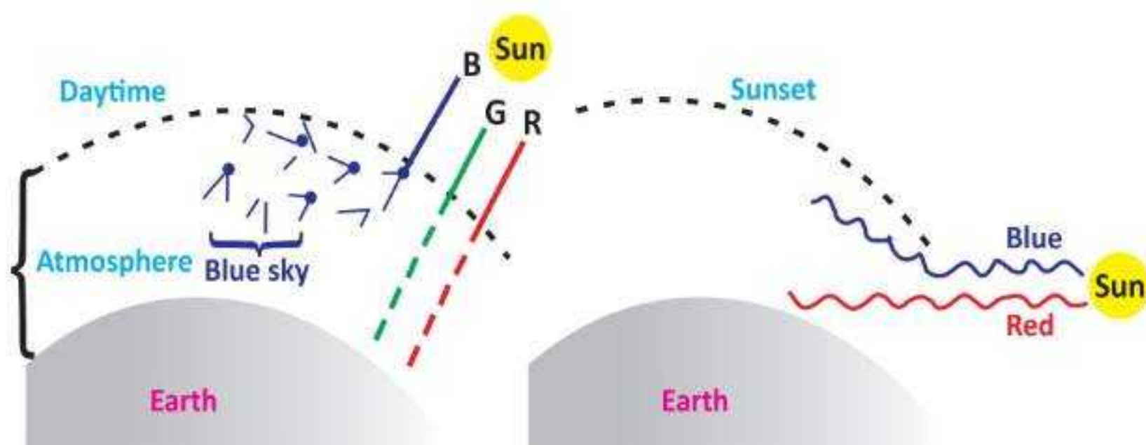
Fig. 18.13: Scattering of sunlight during daytime and sunset
