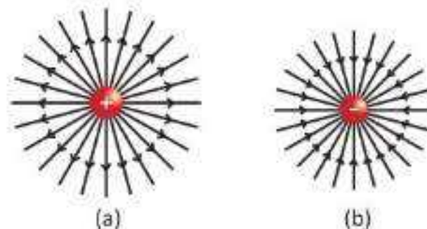
Fig. 15.14: Electric field lines for isolated positive and negative point charges
