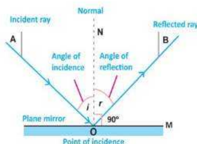
Fig. 14.1: Reflection of light
