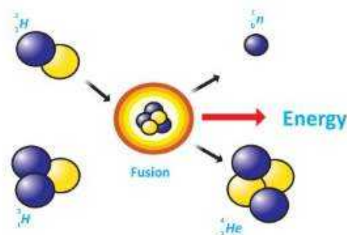
Fig. 20.12: Nuclear fusion reaction
