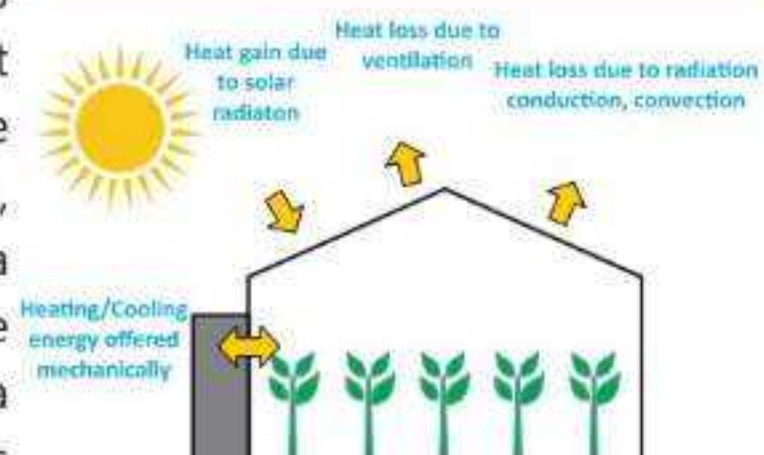
Fig. 11.17: Heat transfer mechanisms in a greenhouse
