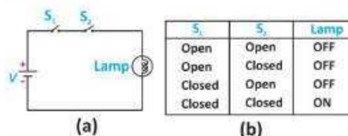
Fig. 19.12: (a) Circuit representation of AND logic using switches (b) Truth table for AND logic
