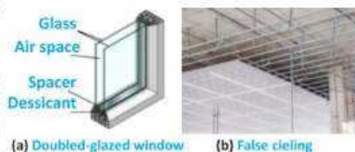
Fig. 11.16: Reducing thermal energy transfer
