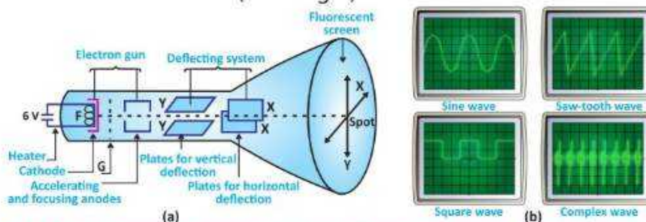
Fig. 18.11: (a) Schematic diagram of CRO (b) Different waveforms displayed on a CRO screen
