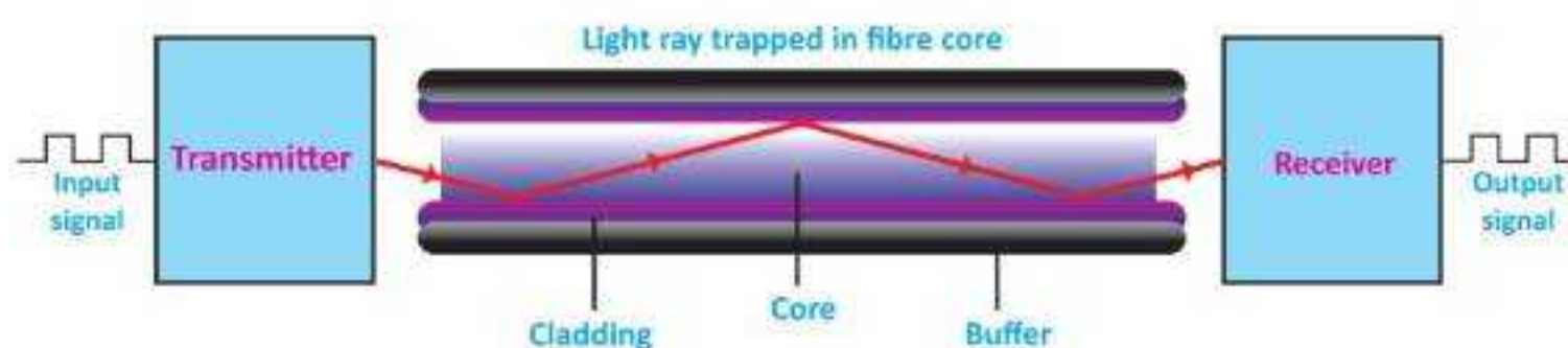
Fig. 14.11: Transmission of information through optical fibre
