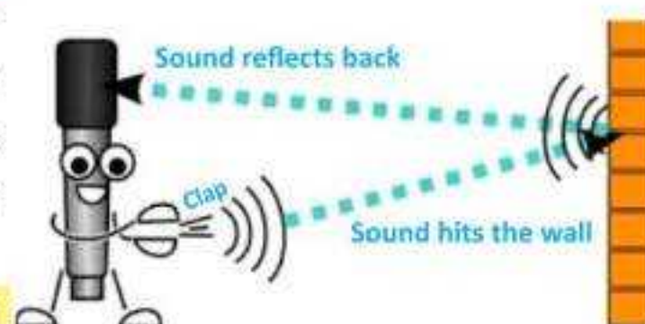
Fig. 13.10: Reflection of sound
