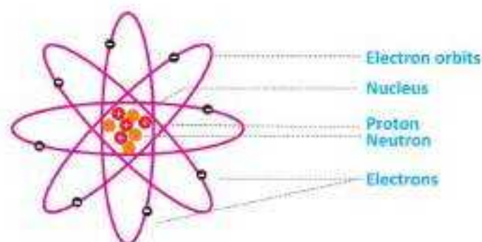
Fig. 20.2: Diagram of an atom showing the nucleus, protons, neutrons, and electron orbits
