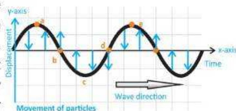
Fig 12.1: Vibration of particles in a wave perpendicular to the wave direction
