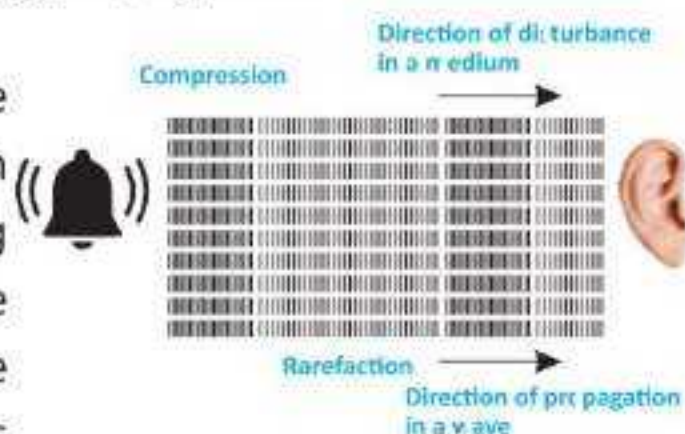
Fig. 12.9: A longitudinal sound wave showing compressions and rarefactions
