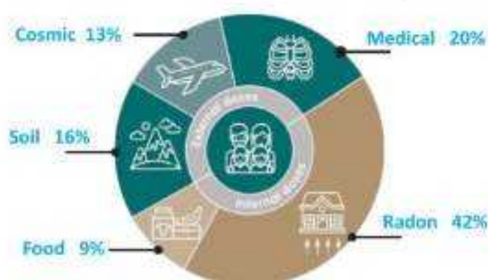
Fig. 21.9: Sources of radiation
