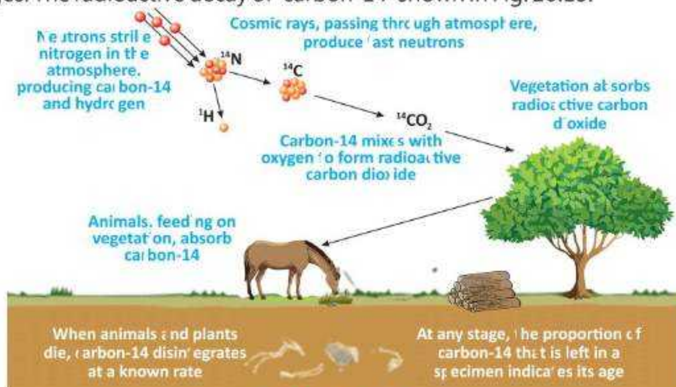
Fig. 20.15: Carbon dating
