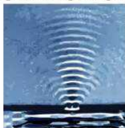
(b) Size of slit is the same as the wavelength of the water waves
