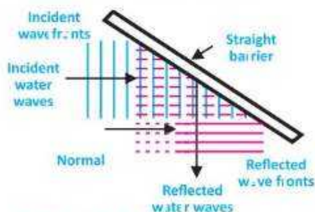
Fig. 12.11: Reflection of water waves
