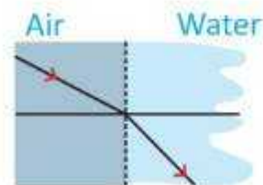
Fig.13.12: Refraction of sound
