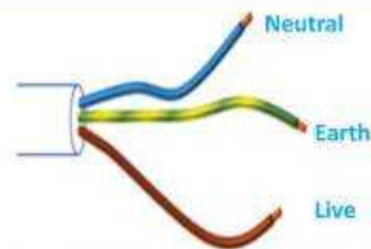
Fig. 16.22: Main circuit wires
