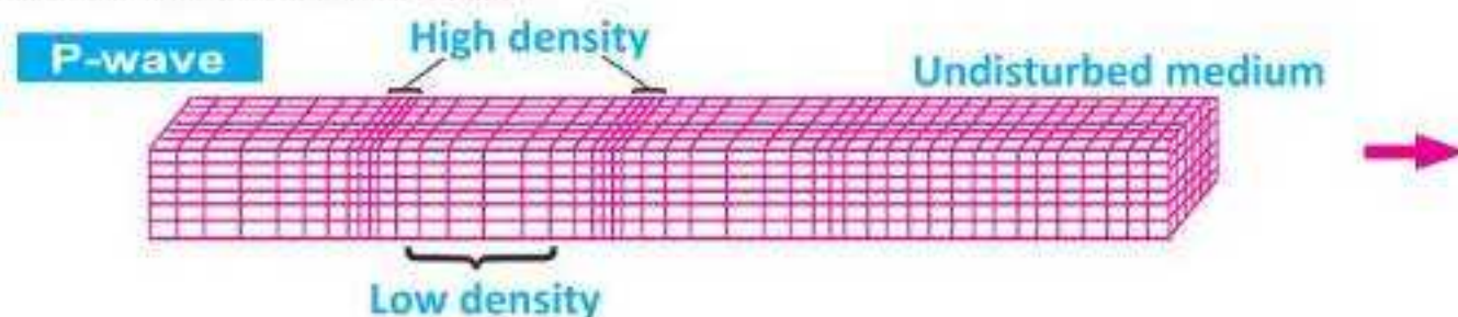
Fig. 12.14: P-wave showing longitudinal motion
