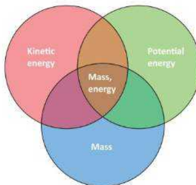
Fig. 20.13: Interconversion of different energies
