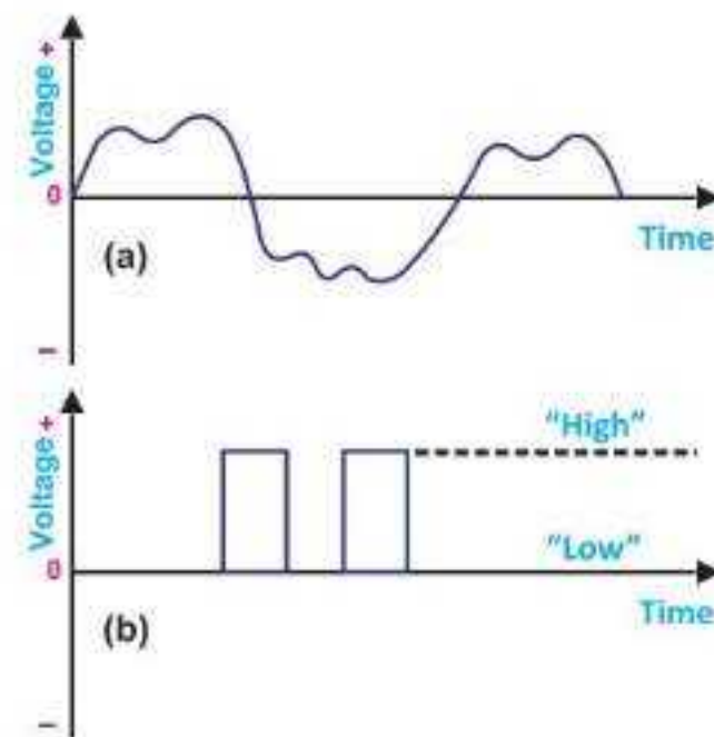
Fig. 19.8: Comparison of analog and digital signals: (a) analog signal varies continuously over time, while (b) digital signal switches between discrete "high" and "low" levels
