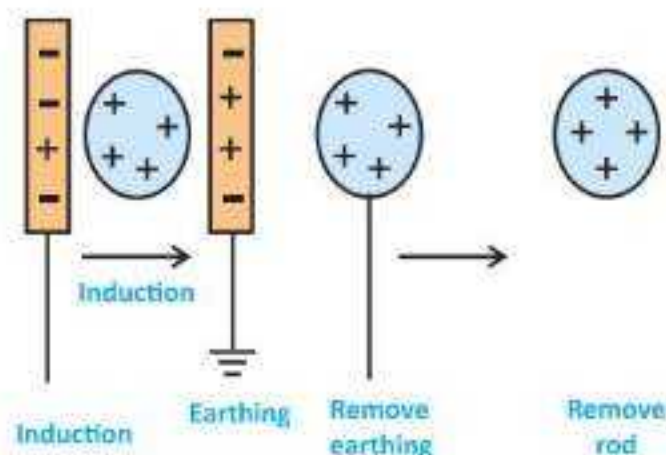
Fig. 15.6: Charging a conductor by induction and earthing
