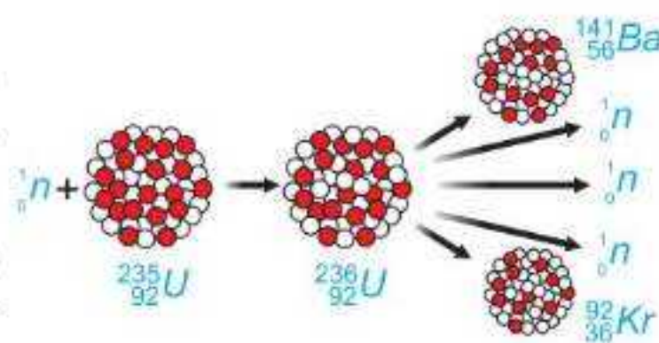
Figure 20.11: Nuclear fission reaction
