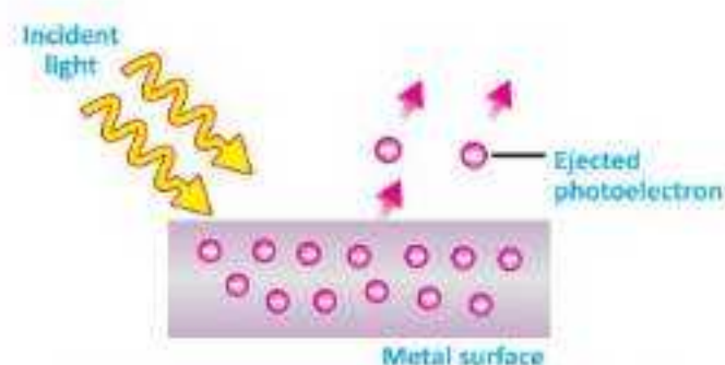
Fig. 18.14: Particle nature of light
