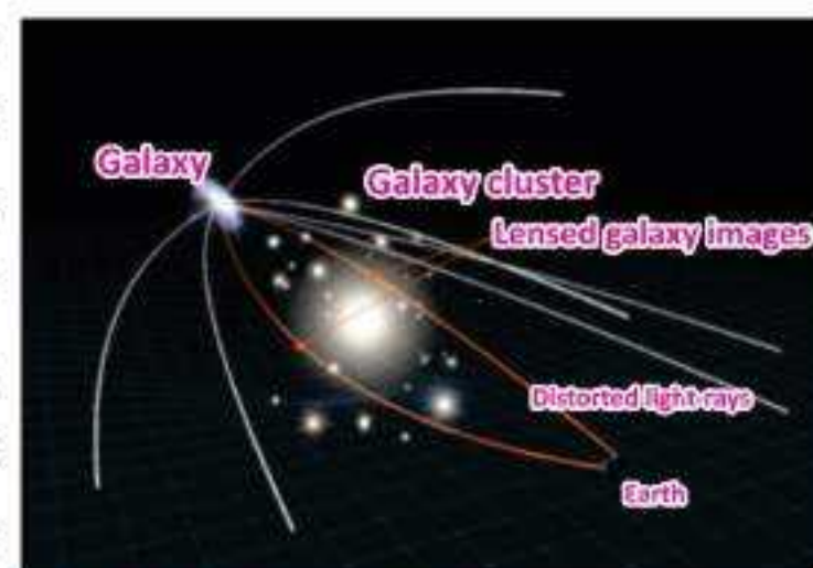
Fig.14.27: Diagram of gravitational lens
