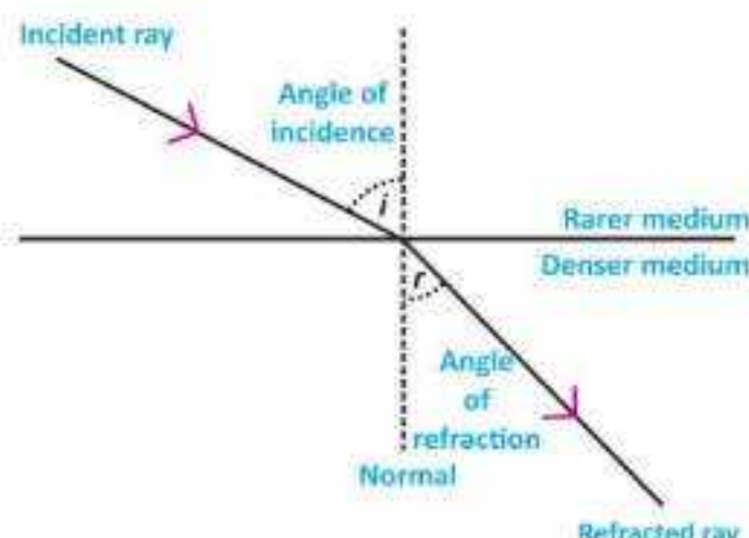
Fig. 14.4: Refraction of light
