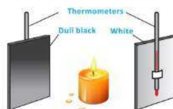
Fig. 11.12: A comparison of absorption of radiations
