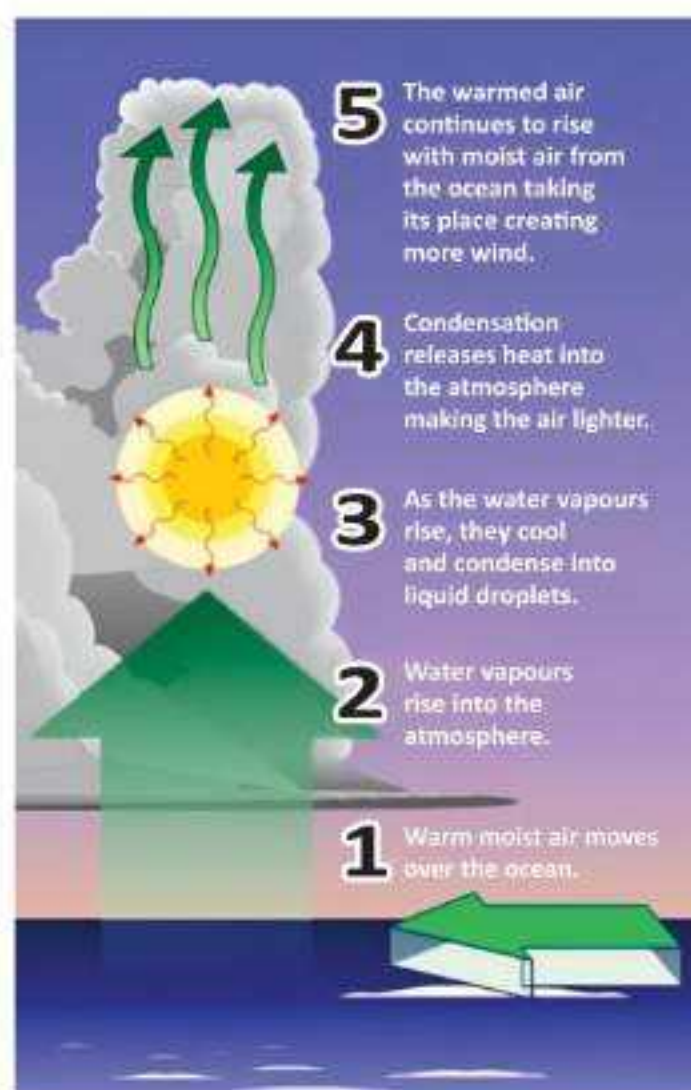
Fig. 21.4: Formation of cyclone
