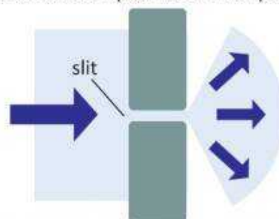
Fig.13.13: Diffraction of sound waves
