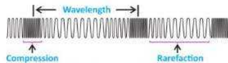
Fig 12.4: Longitudinal wave (Stretched spring)
