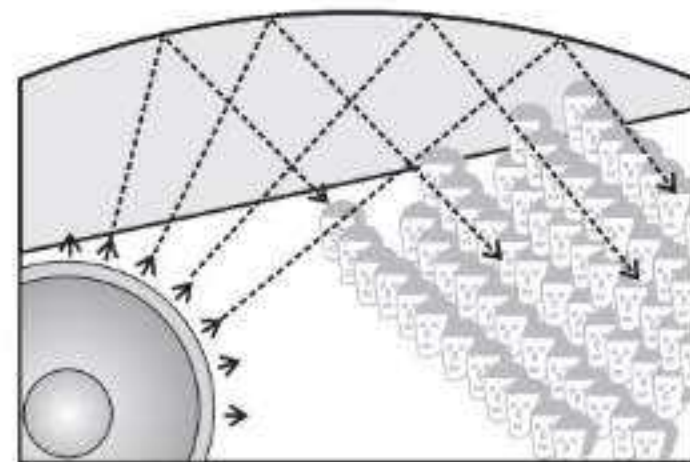
Fig. 13.16(b): Curved ceiling of a conference hall
