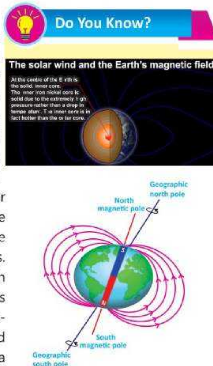
Fig. 17.13: Origin of Earth's magnetic field
