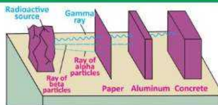
Fig. 20.7: Penetrating power of three types of radiations
