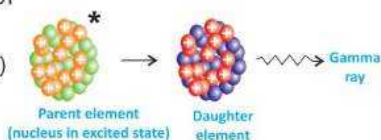
Fig. 20.10: Representing gamma decay
