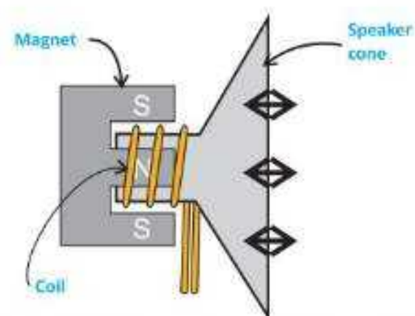
Fig. 17.11: Magnetic effects in loudspeakers
