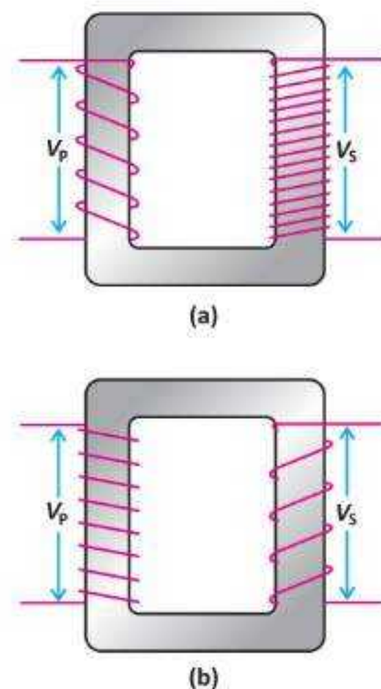
Fig. 18.8: (a) Step-up transformer (b) Step-down transformer
