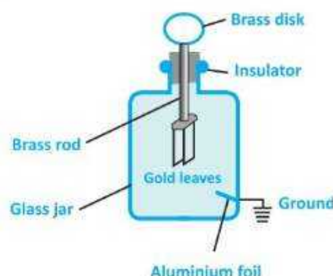
Fig. 15.7: Uncharged electroscope
