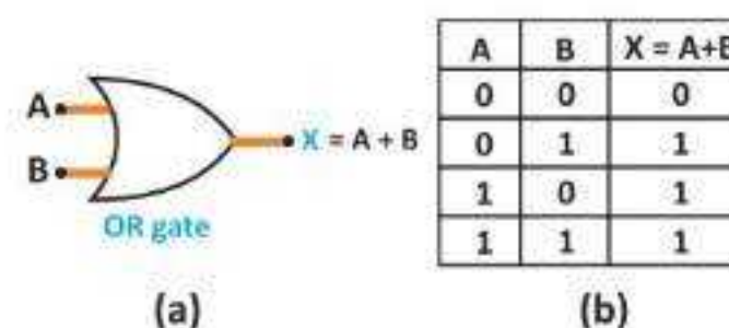
Fig. 19.15: (a) The circuit symbol and (b) Truth table for an OR gate
