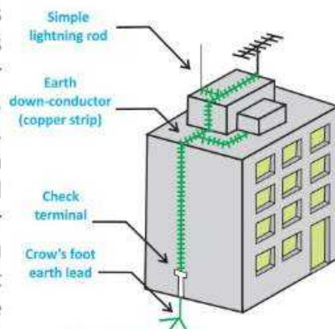
Fig. 15.19: Lightning conductors installed in building
