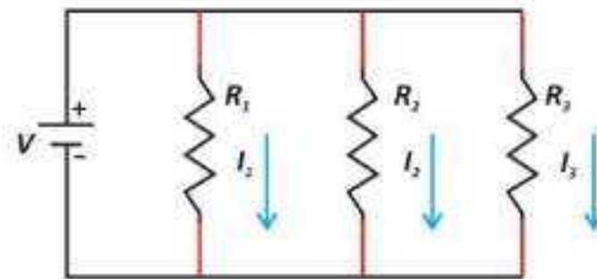
Fig.16.12: Resistors in parallel
