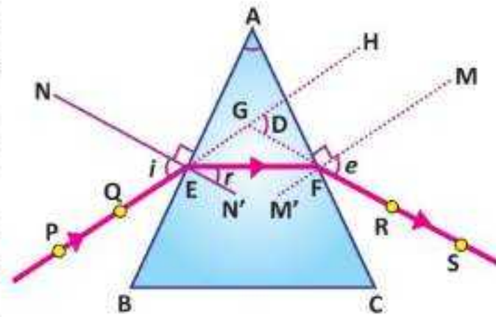
Fig. 14.6: Refraction through a triangular glass prism
