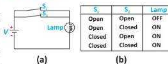
Fig. 19.13: (a) Circuit representation of OR logic using switches (b) Truth table for OR logic
