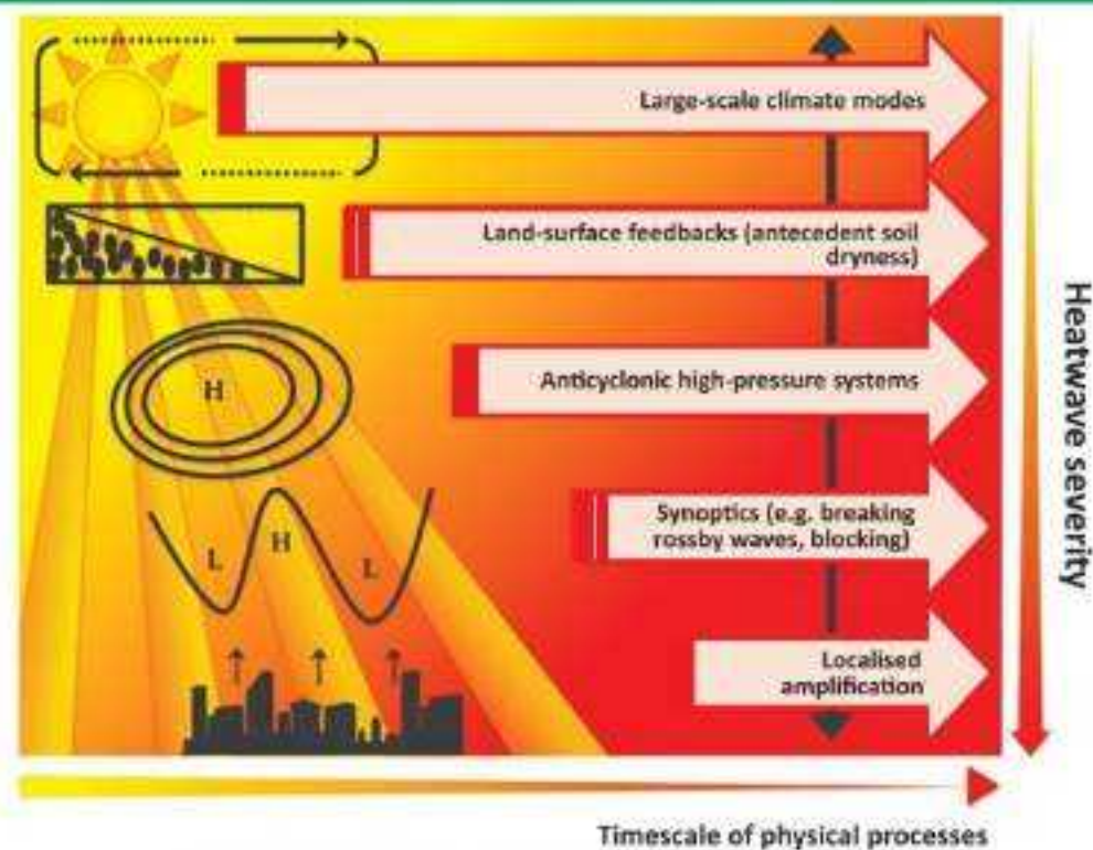
Fig. 21.7: Heatwave schematic illustrating the various physical processes
