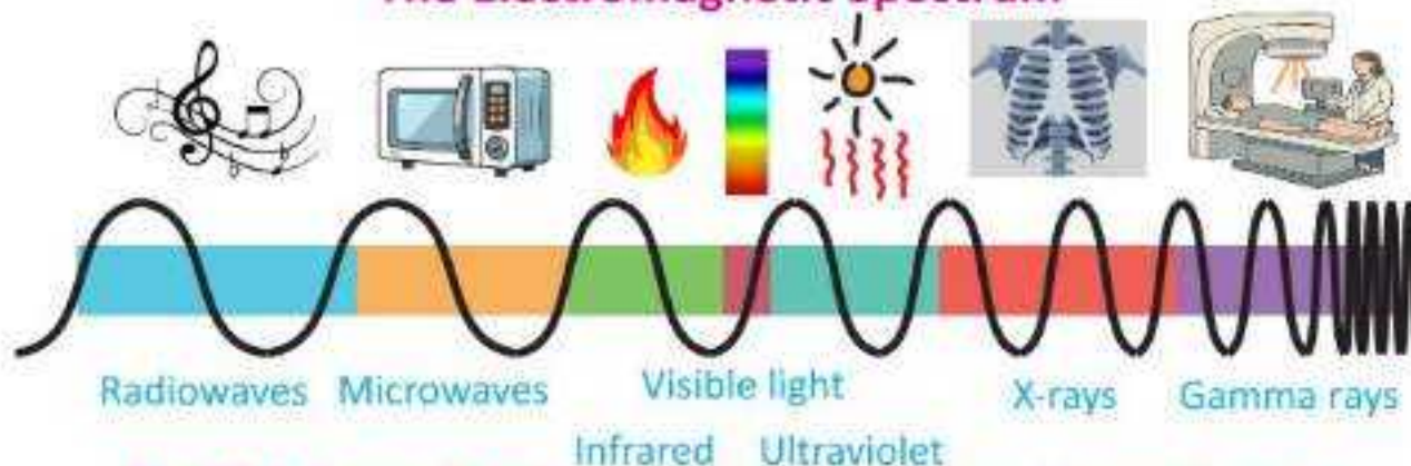
Fig. 12.7: Types of electromagnetic waves arranged by wavelength
