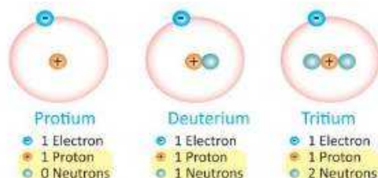
Fig. 20.3: Isotopes of hydrogen
