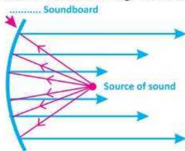
Fig. 13.16(a): Soundboard used in a big hall
