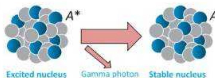
Fig. 20.6: Representing gamma radiation
