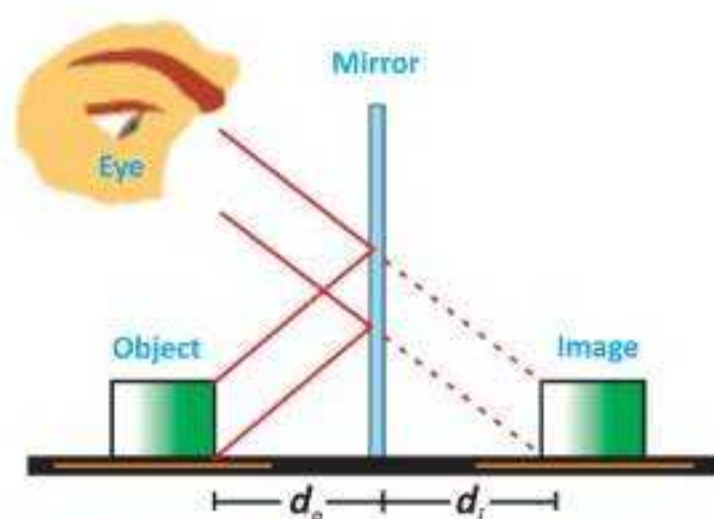
Fig. 14.2: Image formation by a plane mirror
