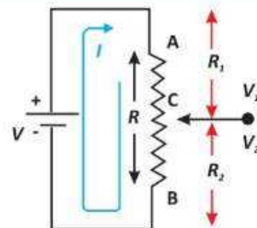
Fig.16.15: Potential divider circuit
