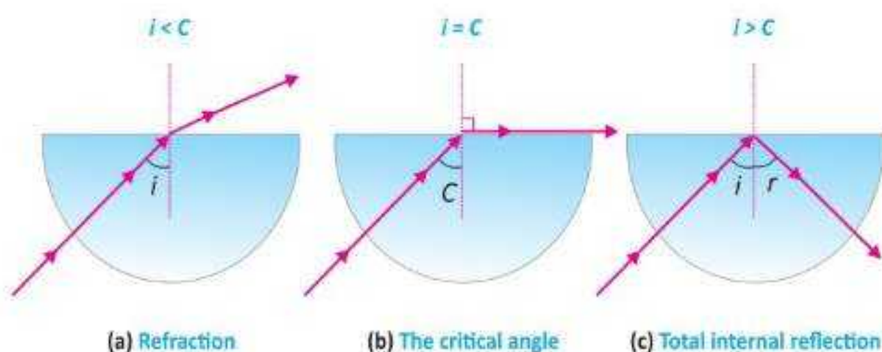
Fig. 14.9: Experiment for total internal reflection
