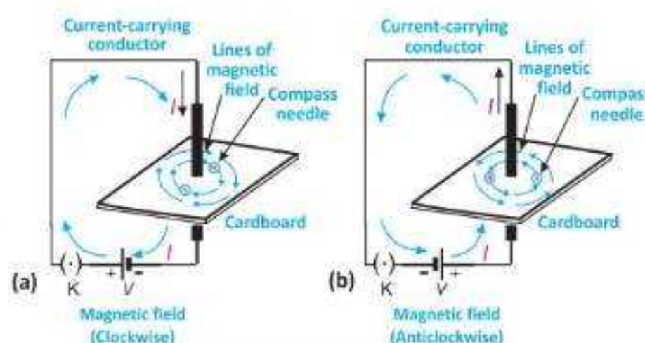
Fig. 17.1: Magnetic effects of a current
