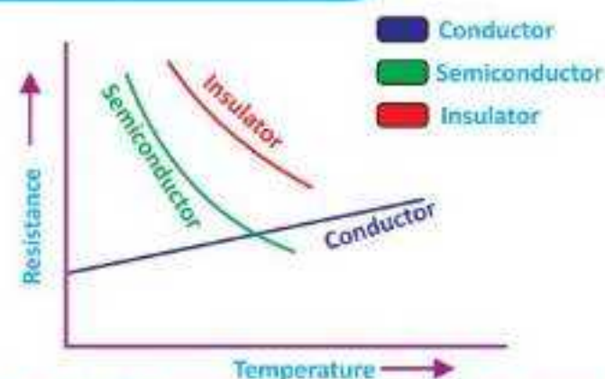
Fig.16.14: Temperature effect on materials
