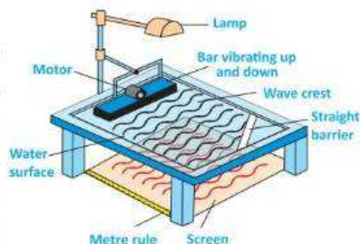
Fig. 12.10: Ripple tank setup showing water waves
