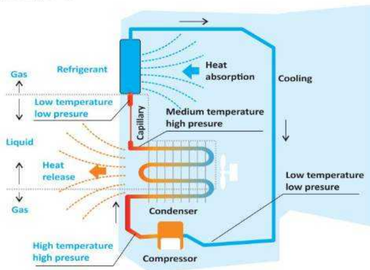
Fig. 10.11: Block diagram of refrigerator
