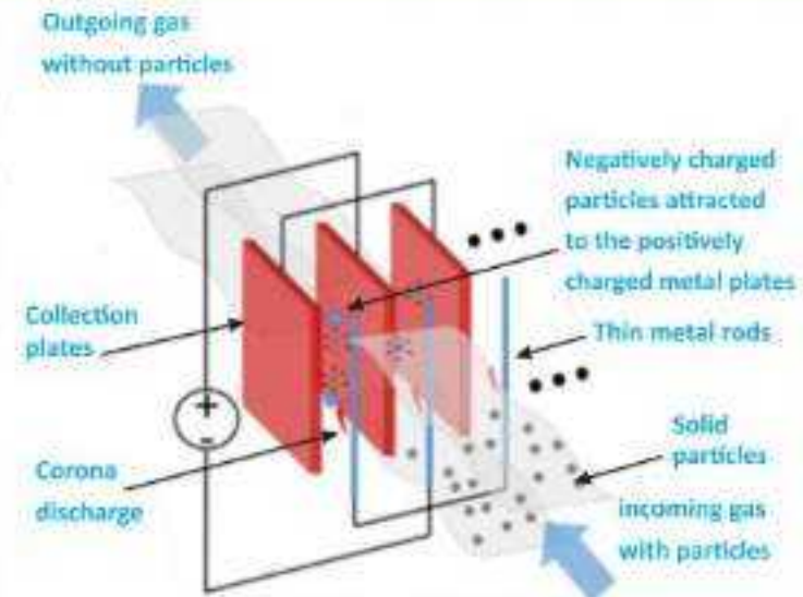
Fig. 15.11: Electrostatic precipitator The diagram of an electrostatic precipitator is shown in Fig. 15.11.
