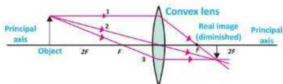
Fig. 14.18: Real image formation by a converging lens
