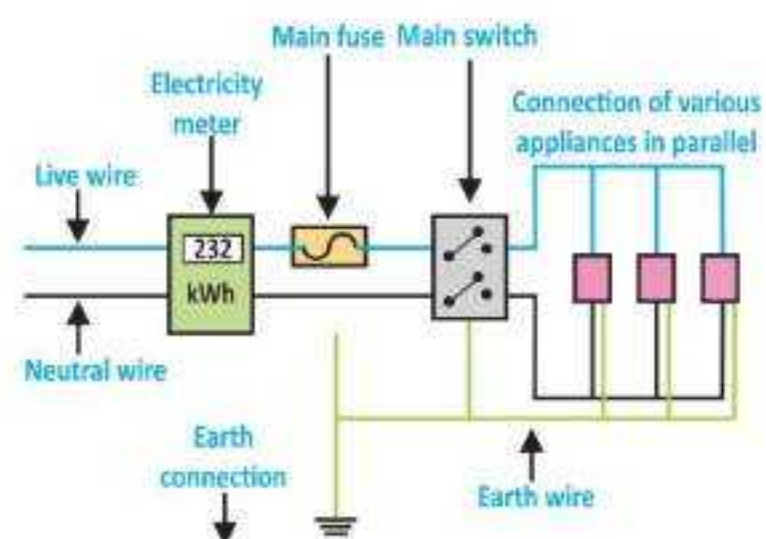
Fig. 16.19: Household circuit
