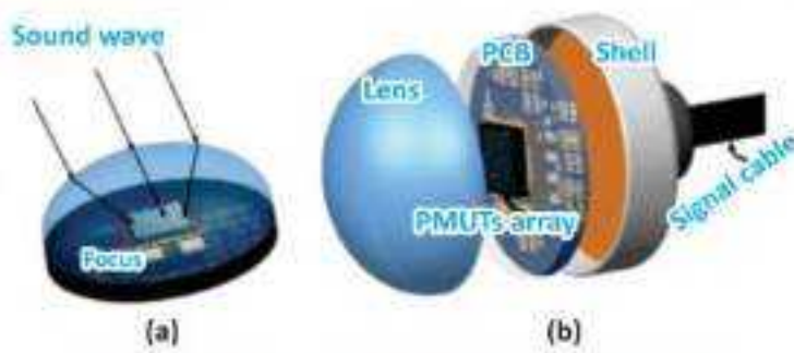
Fig. 14.28: Diagram of acoustic lens
