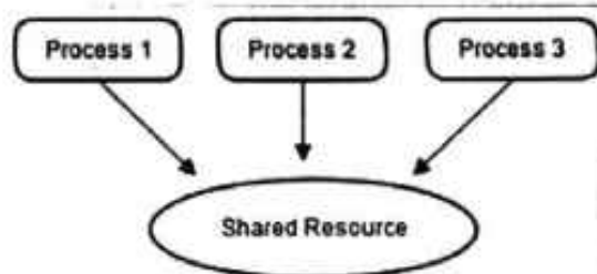
Fig.1.22: Process Synchronization
