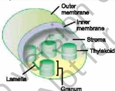
Figure 6.6: Structure of Chloroplast
