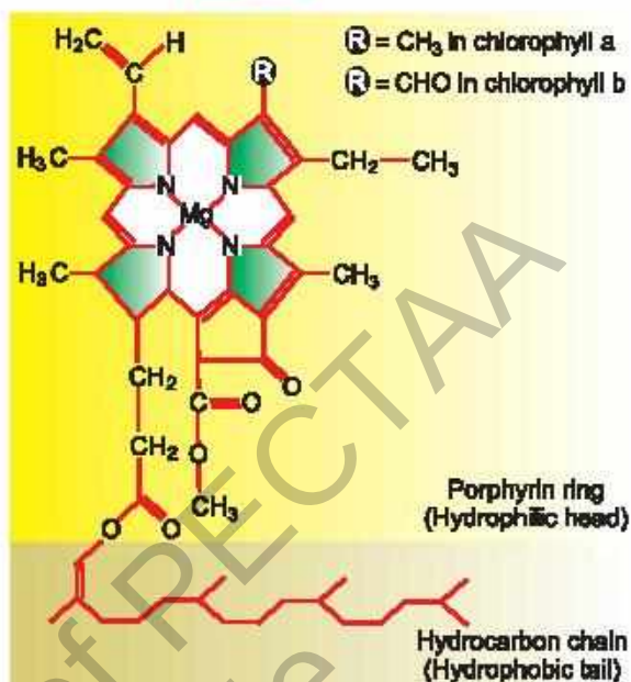
Figure 6.4: Molecular structure of chlorophyll a and chlorophyll b
