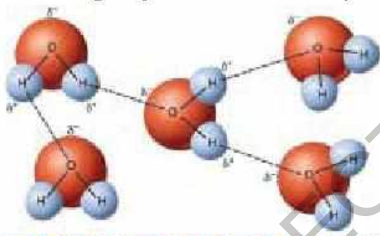
Figure 4.3: Hydrogen bond between water molecules
