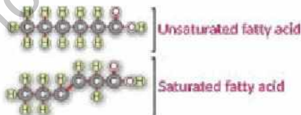
Figure 4.32 Fatty acids
