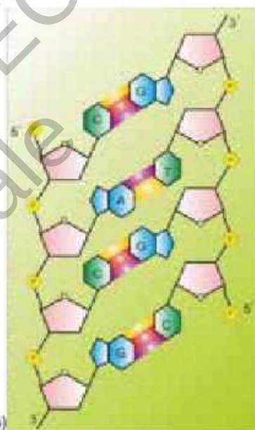
Figure 4.44: (a) Watson and Crick model of DNA, (b) The detailed structure of DNA
