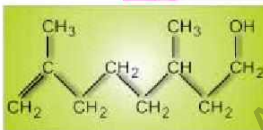
Figure 4.36: Structure of terpenes
