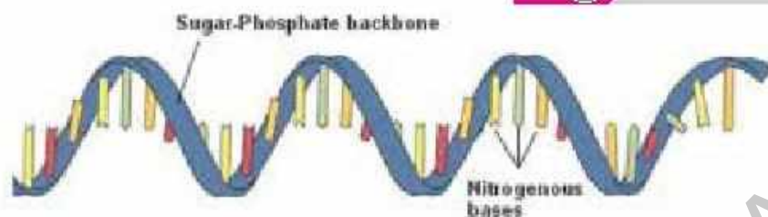
Figure 4.45: A model of DNA structure
