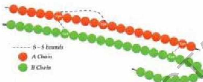
Figure 4.27: Chains of Insulin
