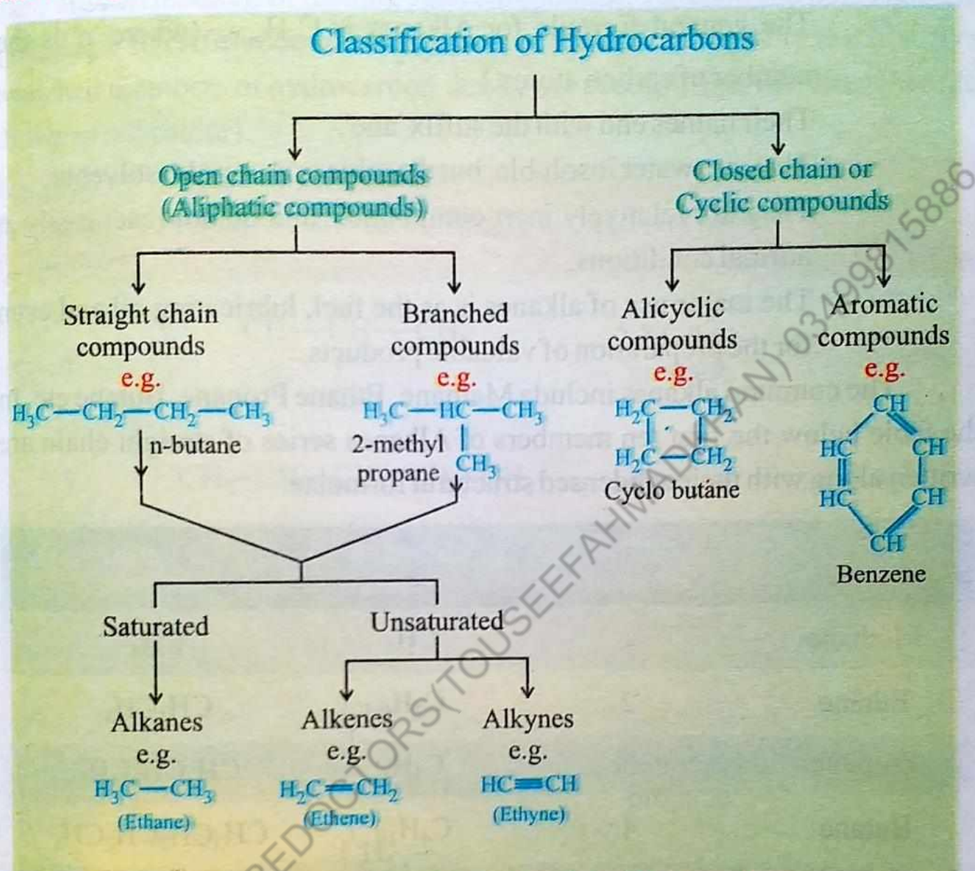
Fig. 12.5: Flow chart of classification of Hydrocarbons
