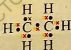
Fig. 12.8: Structure of Ethane Molecule
