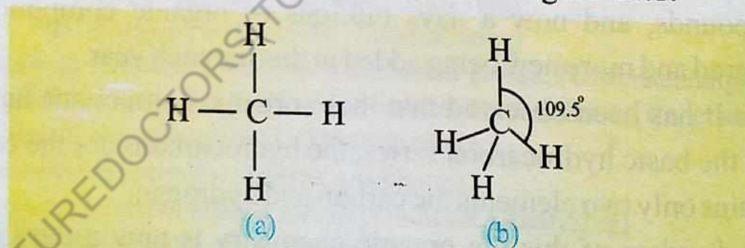
Fig. 11.1: Two dimensional representation of \text{CH}_4 molecule, (a) general representation, (b) Representation showing angles
