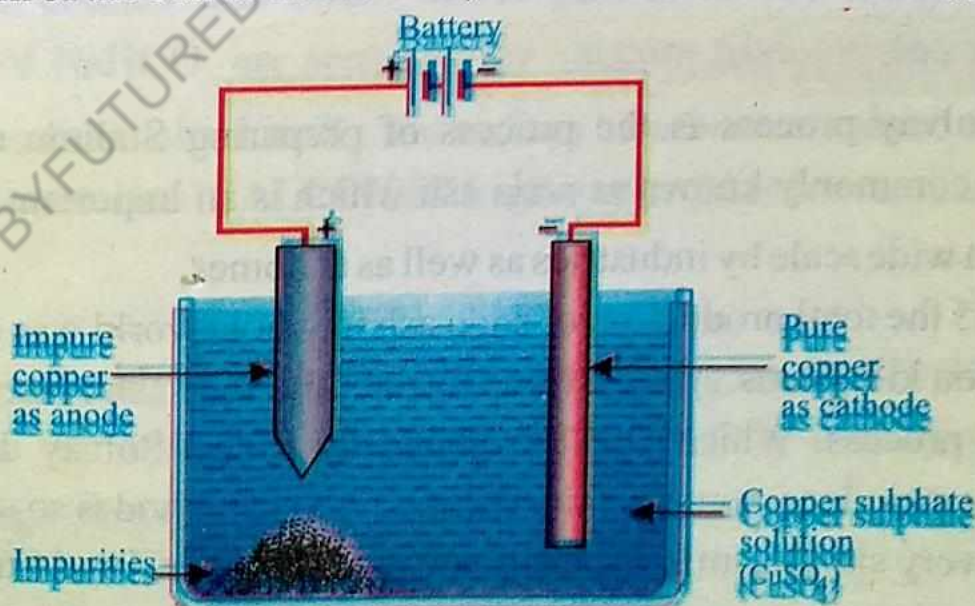
Fig. 16.1: Experimental set up for the electrolytic refining of copper :
