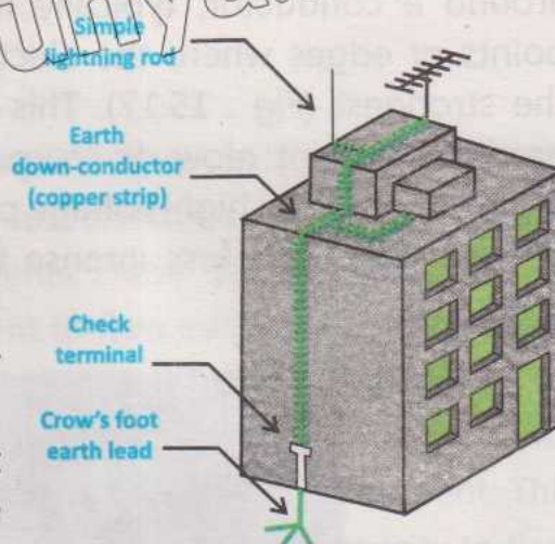
Fig. 15.19: Lighting conductors installed in building
