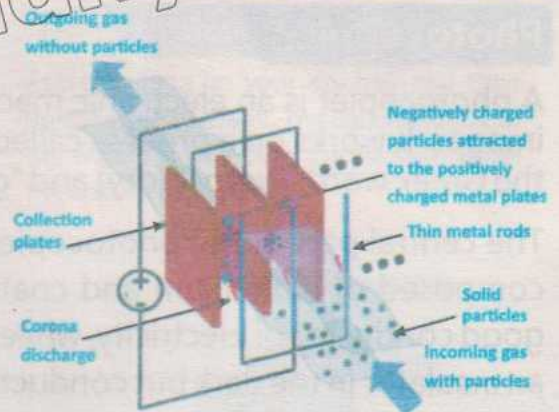
Fig. 15.11: Electrostatic precipitator
