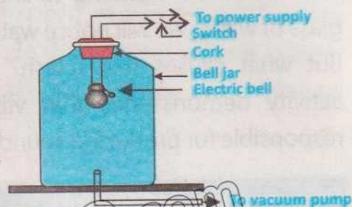
Fig. 13.5: Bell jar apparatus
