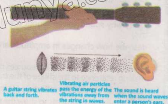
Fig. 13.1: Vibrations of guitar strings produce sound waves
