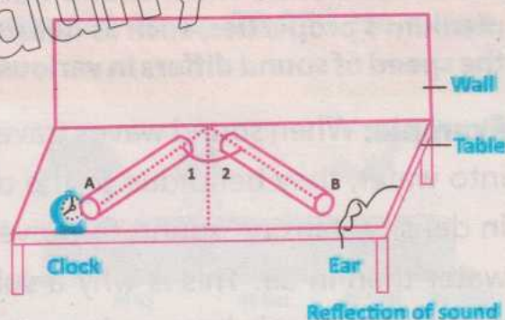
Fig.13.11: Reflection of sound using plastic tubes and a ticking clock
