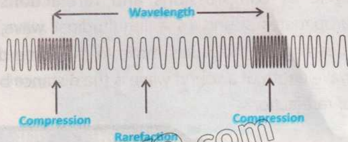
Fig. 13.6: Propagation of longitudinal sound waves in a slinky, showing compressions and rarefactions
