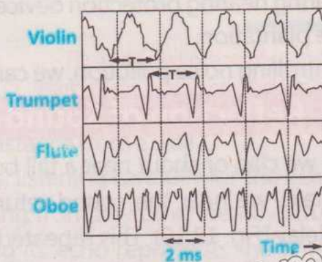
Fig. 13.9: Oscilloscope traces of different sound sources
