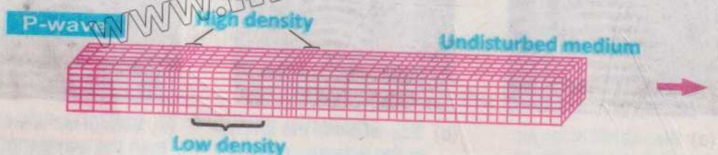
Fig. 12.14: P-wave showing longitudinal motion
