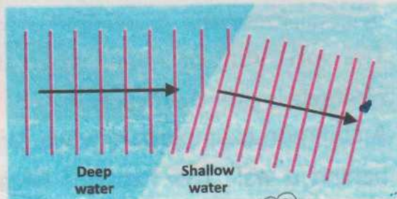
Fig. 12.12: Refraction of waves
