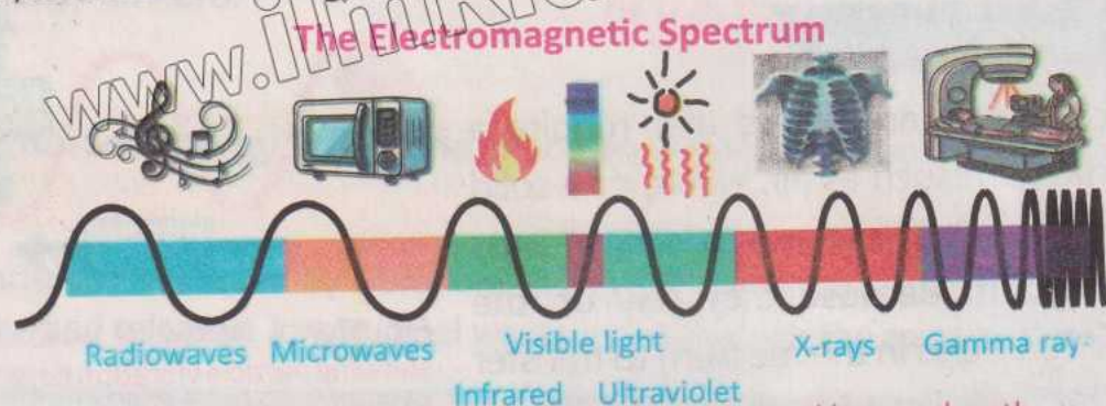
Fig. 12.7: Types of electromagnetic waves arranged by wavelength
