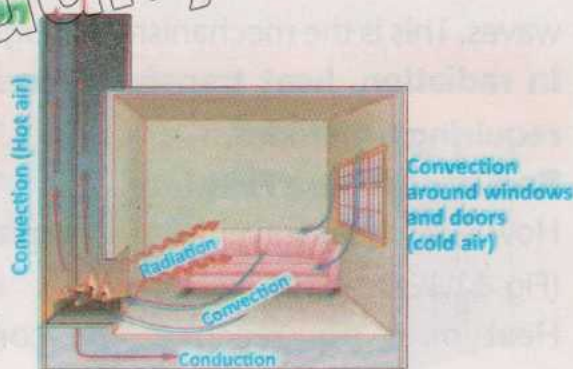
Fig. 11.8: Heating room by convection
