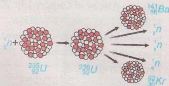
Figure 20.11: Nuclear fission reaction
