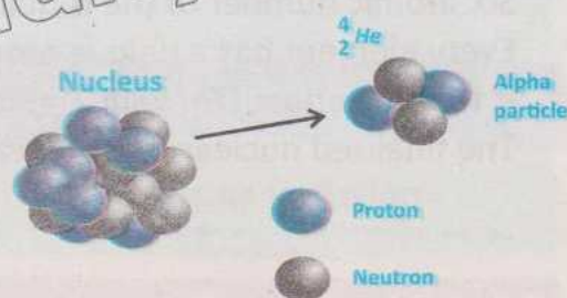
Fig. 20.9: Representing alpha decay
