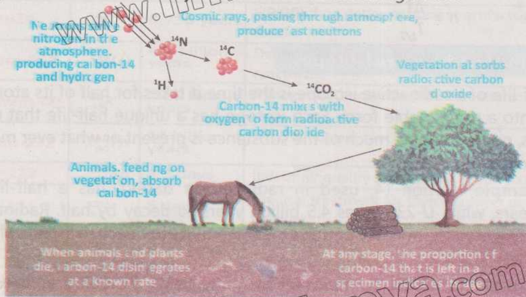
Fig. 20.15: Carbon dating
