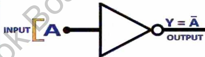
Fig. 6.6 NOT Gate
