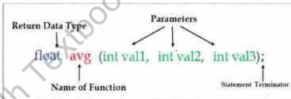
Fig. 5.1 Function Declaration
