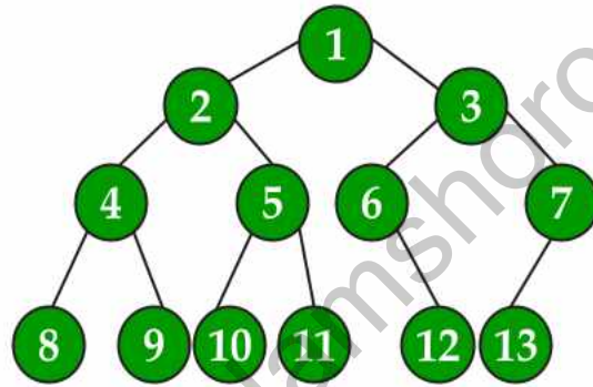
Fig. 1.6: Tree Data Structure
