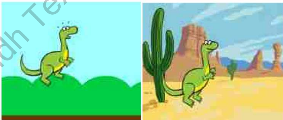
Fig. 7.15 Changing Backdrop
