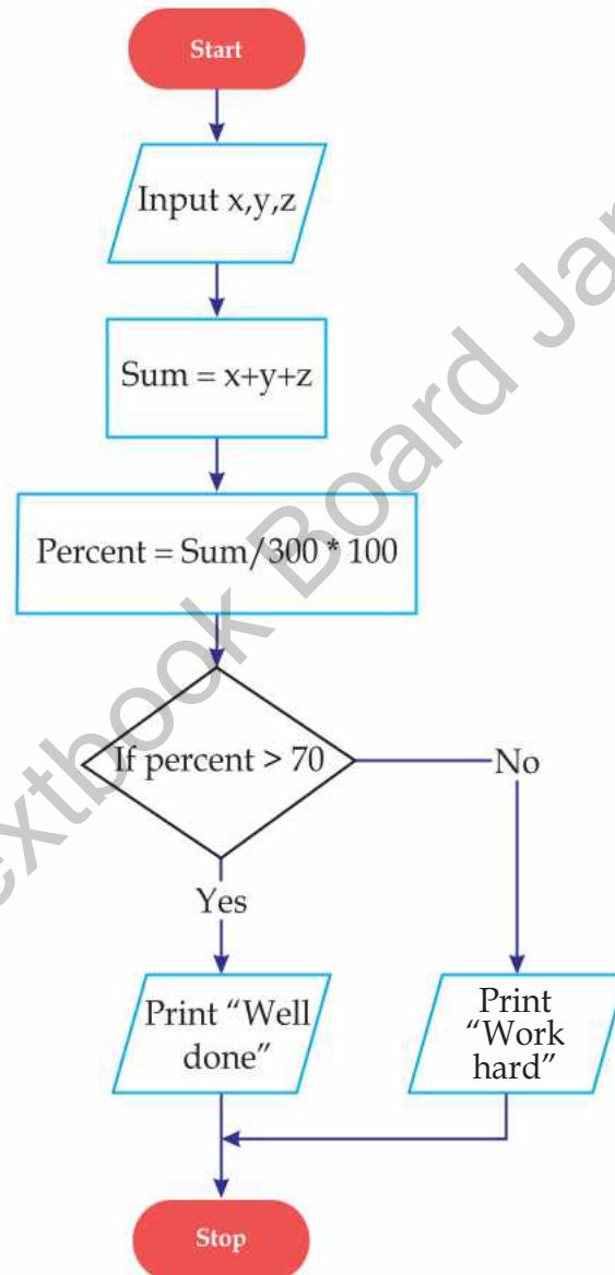
Fig. 1.2: Sample Flowchart
