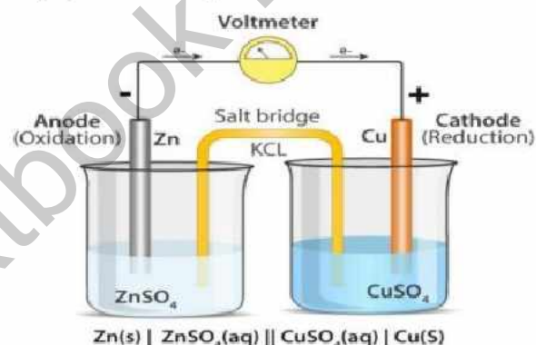
Figure 7.19 Electrochemical cell
